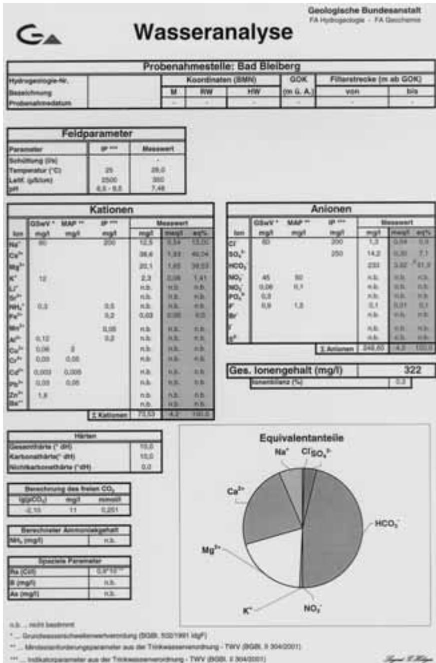
Figure 11- Hydrochemical composition
