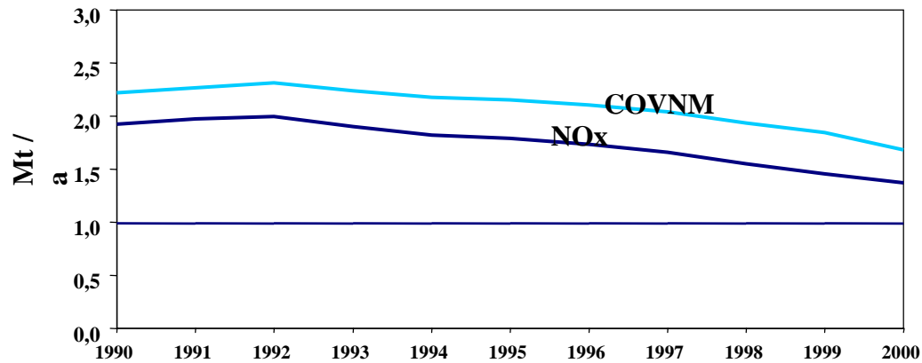
National NOx and COVNM emissions, 1990-2000
