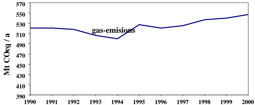
National greenhouse gas emissions, 1990-2000
