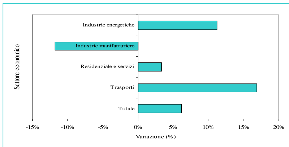
Per cent variation of greenhouse gas emissions for economic sector, 1990-2000
