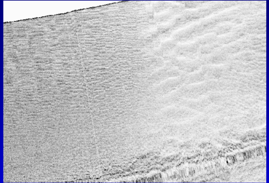
Megaripple e sand waves
