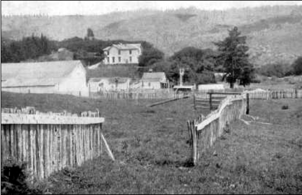
Figure c – April 18, 1906, San Francisco earthquake ( M_s 8.3): 8.5 feet of right-lateral fault movement northwest of Woodville, California. Photo G.K. Gilbert.
