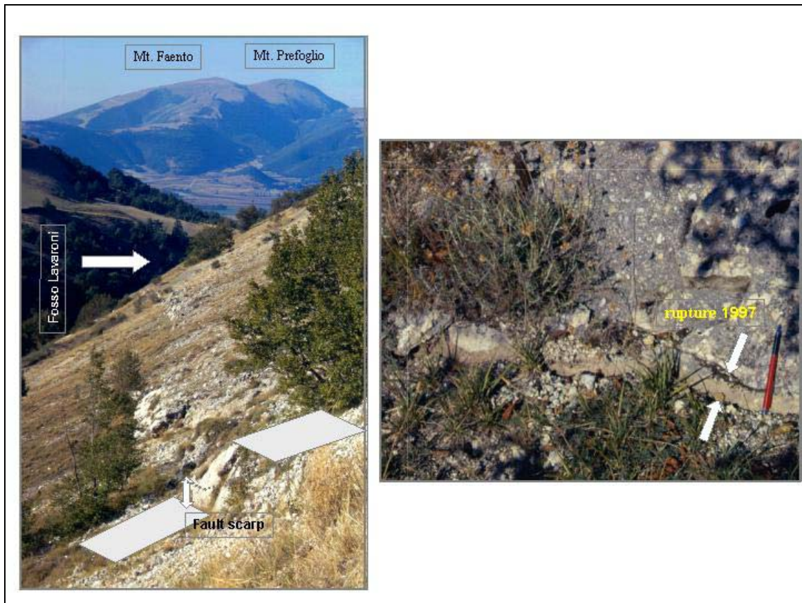
Figure o – Fault rupture of the September 26, 1997 earthquake ( M_w 6) in Umbria-Marche region (central Italy); Vittori et al., 2000. Photo E. Vittori.
