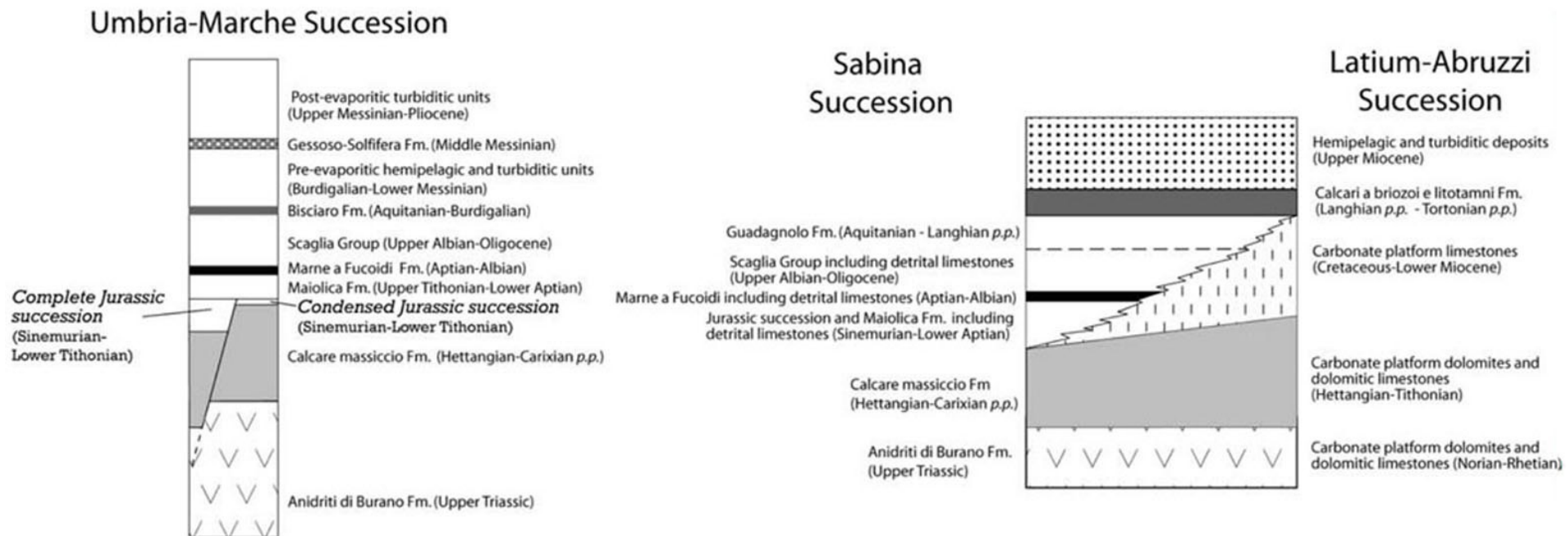
Fig. 2 - Schematic stratigraphic column (left) for the Umbria-Marche basin succession, and (right) stratigraphic relationships between Latium-Abruzzi carbonate platform and slope-to-basin Sabina (Gran Sasso) transitional successions (from Mazzoli et al., 2005).
