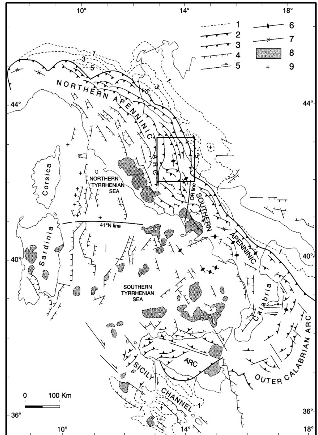
Fig. 1 - Structural map of Apennines and Tyrrhenian Sea. Legend: 1) base of Pliocene/Quaternary isobaths (in kilometres); 2) front of thrust belt; 3) major post-Tortonian thrusts; 4) normal faults; 5) strike-slip faults; 6) antiforms; 7) synforms; 8) volcanoes; 9) intrusive bodies. OR line: Ortona-Roccamonfina line. Square indicates central Apennines area shown in fig. 3. Modified after Patacca et al. (1993).
