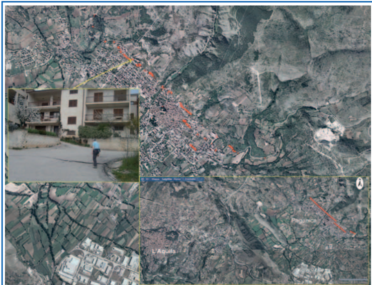
Figure 7.4: Surface rupture of the Paganica fault 5
