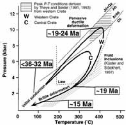
Figure 6 - Pressure-temperature-time (P-T-t) loop of the Phyllite-Quartzite unit of Crete, taken from Thomson et al. (1998). Ab-albite, Arag-argonite, Cc-calcite, Jd-jadeite, Qtz-quartz, Law-lawsonite.
