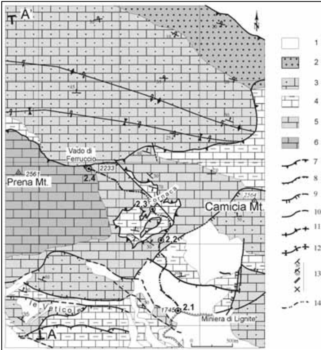
Figure 2.1 - Geological-structural sketch of the Prena Mt.- Camicia Mt. area. The location of the area is shown in Figure 1.1. 1) Quaternary deposit; 2) Calcareni glauconitiche-Marne con cerroghna (Lower-Upper p.p. Miocene); 3) Maiolica-Scaglia Cinerea (Lower p.p. Cretaceous- Middle Eocene); 4) Corniola-Calcari bioclastici inferiori (Middle Lias - Malm); 5) Dolomie Bituminose - Calcari dolomitici (Upper Trias - Lower Lias); 6) Dolomia Principale (Upper Trias); 7) Thrust; 8) Normal fault; 9) Low-angle normal fault; 10) Fault; 11) Anticline; 12) Syncline; 13) Bedding; 14) Itinerary and location of the stops (2.1 - 2.4); A-A': trace of geological section across Prena Mt. (Figure 2.2).
