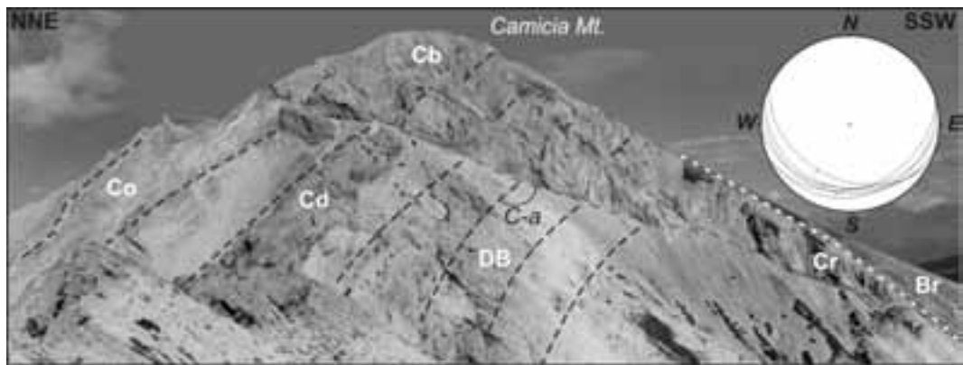
Figure 2.10 - The Camicia Mt. low-angle normal fault and relative synthetic fault planes. DB: Dolomie Bituminose (Upper Triassic); Cd: Calcarei Dolomitici (Lower Lias); Co: Corniola (Middle Lias); Cbs: Calcarei bioclastici superiori (Lower Cretaceous); Cb: bioclastic Calcareenites (Cretaceous-Oligocene); Br: continental breccia (Quaternary); C-a: Cut-off angle. The stereonet shows the geometry and kinematics of the fault.
