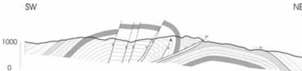
Figure 3.11 - Structural sketch of the Sibillini Mts 1) Thrust; 2) Laga Detachment; 3) Normal fault; 4) Anticline axial trace; 5) Syncline axial trace; 6) Blind up-thrust; 7) Hemipelagic and siliciclastic succession (Upper Miocene): Marne con cerrogna-Laga Fm.; 8) Pelagic and hemipelagic succession (Cretaceous-Oligocene): B- Marne a Fucoidi, C- Scaglia Cinerea; 9) Pelagic succession (Lower Lias-Cretaceous p.p.); 10) Carbonate platform (Lower Lias): Calcare Massiccio Fm.; 11) Evaporites and dolomites (Triassic): Anidriti di Burano Fm.; 12) Itinerary and location of the stops (3.6 - 3.7); A-B: trace of cross-section in Figure 3.12. a) Stratigraphic column: A- Pelagic condensed succession
