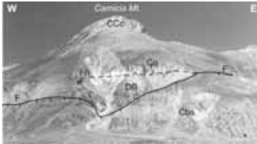
Figure 1.10 - Detail showing the Camicia Mt. low-angle normal fault (Fn), and the Campo Imperatore high-angle normal faults (F). DB: Dolomie Bituminose; Co: Corniola; Cbs: Calcarei bioclastici superiori; CCC: Scaglia/Cretaceous clastic limestones.
