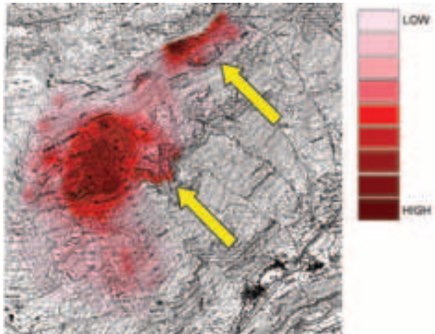
Figure 42 - Hazard map of the Clot Brun area
