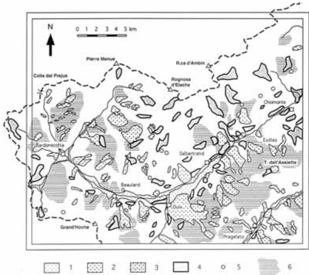
Figure 27 - Quaternary deposits and large-slope instabilities distribution in the area of the “Bardonecchia” sheet of the Geological map of Italy 1:50,000 in scale. 1) lacustrine and alluvial deposits; 2, 3) landslide deposits; 4) glacial and fluvioglacial deposits 5) well cemented heterogeneous deposits; 6) deep-seated gravitational deformations. (from Giardino & Fioraso, 1998).
