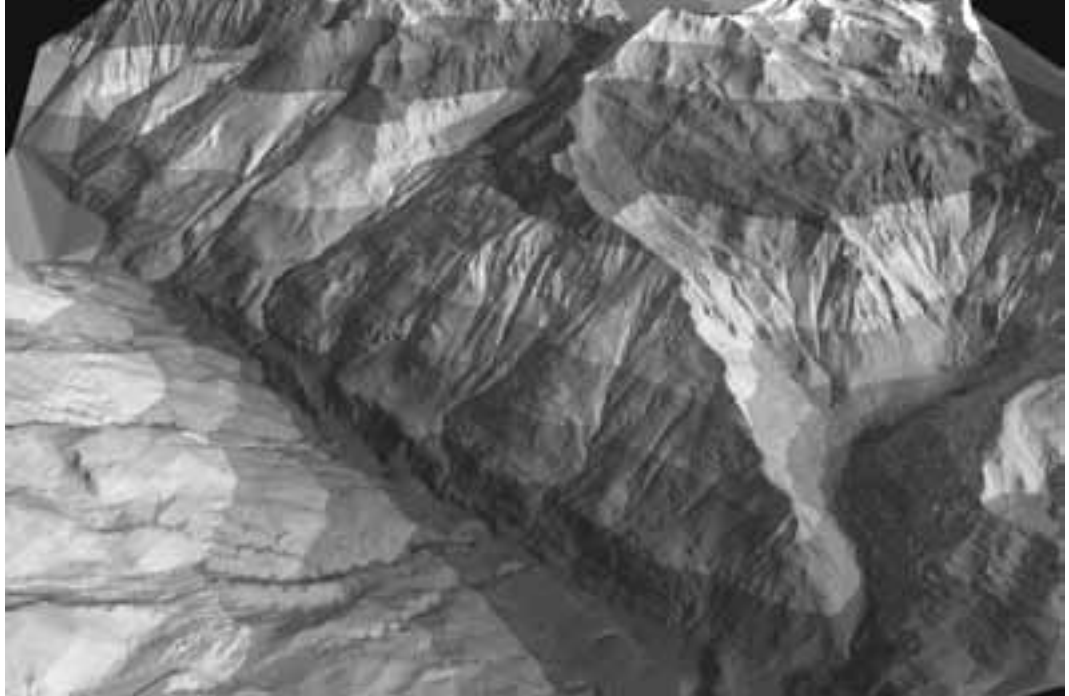
Figure 43 - DEM of the middle Susa Valley with Clot Brun large slope instability (central part of the image, left side of the valley).
