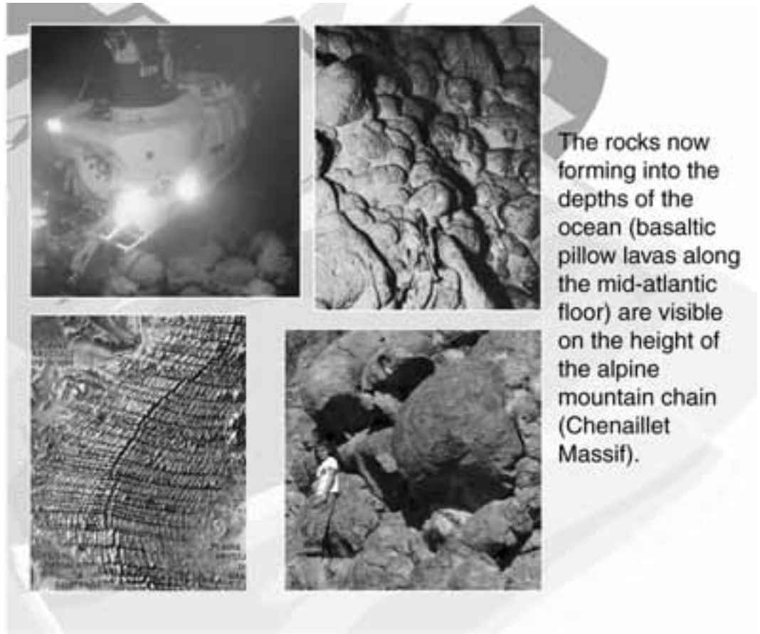
Figure 32 - Images from the “Garden of the Rocks”: discovering the origin pillow lavas (Artwork by Pellegrino P., 2003).
