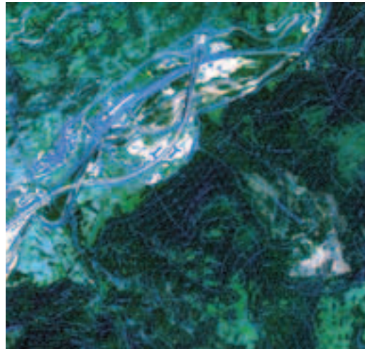
Figure 38 - Cassas Landslide: orthorectified image with reference cartography, scale 1:10.000.
