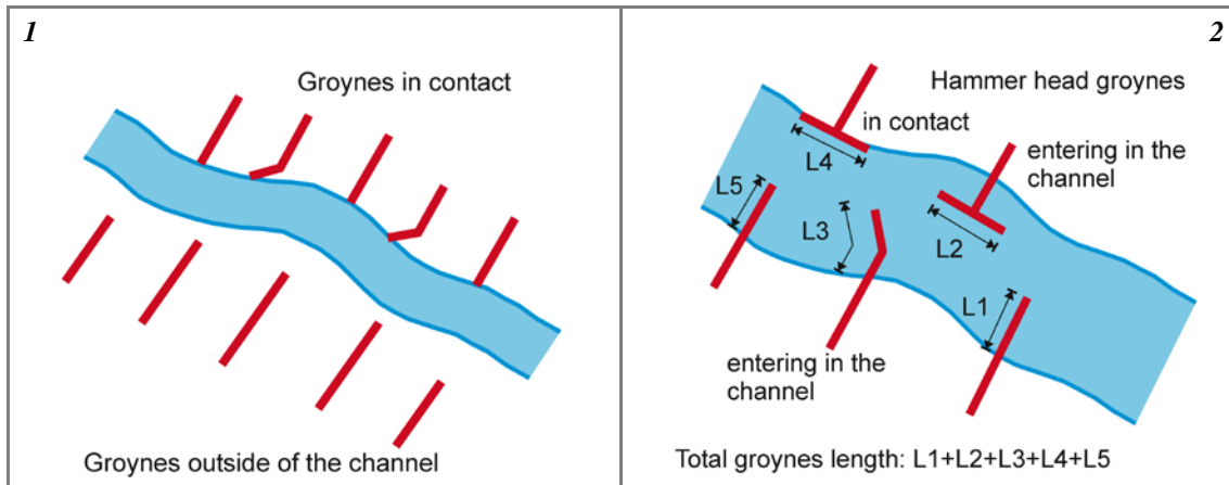
Figure 67 – Case of groynes. (1) Groyne outside of the channel are not considered (instead, they are accounted for in the indicator F5 ); in the case of straight groyne in contact with the channel boundary, the width of the groyne head is usually negligible. (2) In the case of groyne entering in the channel, the greater size between protruding length and head width is considered (the latter is generally the prevailing size in the case of hammer head groyne). Note that hammer head groyne in contact (as opposed to straight or bayonet groyne) are considered.
