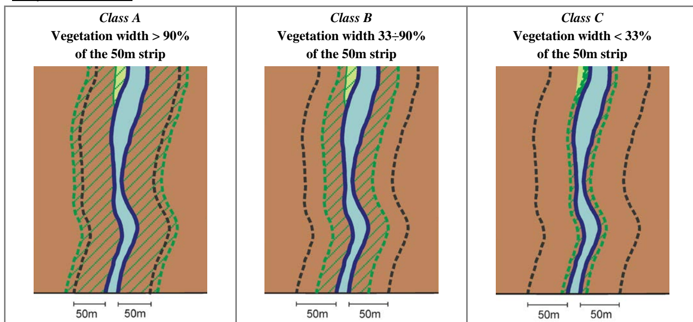
Figure 47 – Width of functional vegetation in confined channels. Class A : the vegetation corridor occupies > 90% of the plain and adjacent hillslopes (for a strip of 50 m for each side, represented by the dotted black line). Class B : the vegetation corridor is between 33 and 90%. Class C : the vegetation corridor is extremely limited (< 33%).
