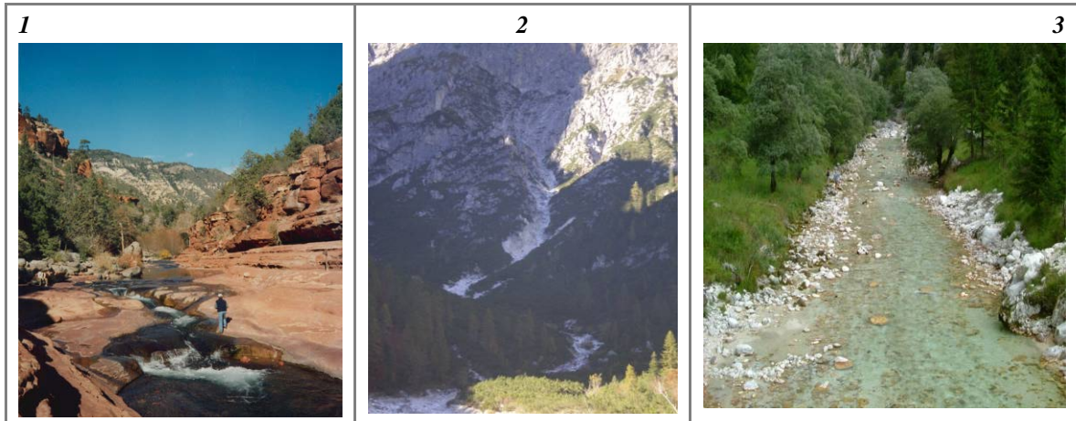
Figure 10 – First morphological classification of streams at reach scale. (1) Bedrock channel; (2) colluvial channel; (3) alluvial (mobile bed) channel.
