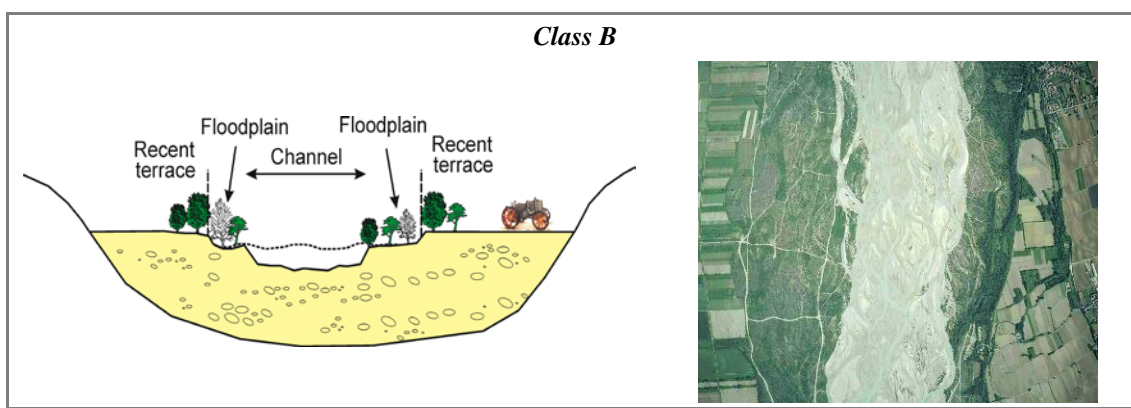
Figure 27 – CASE 3 : the channel is moderately incised and slightly narrowed compared to 1954. Vegetation corridor is continuous and wide ( F12 and F13 in Class A ). Field assessment enables verification that the vegetation corridor also includes portions of “recent” terraces, therefore the floodplain is not sufficiently wide ( Class B ).
