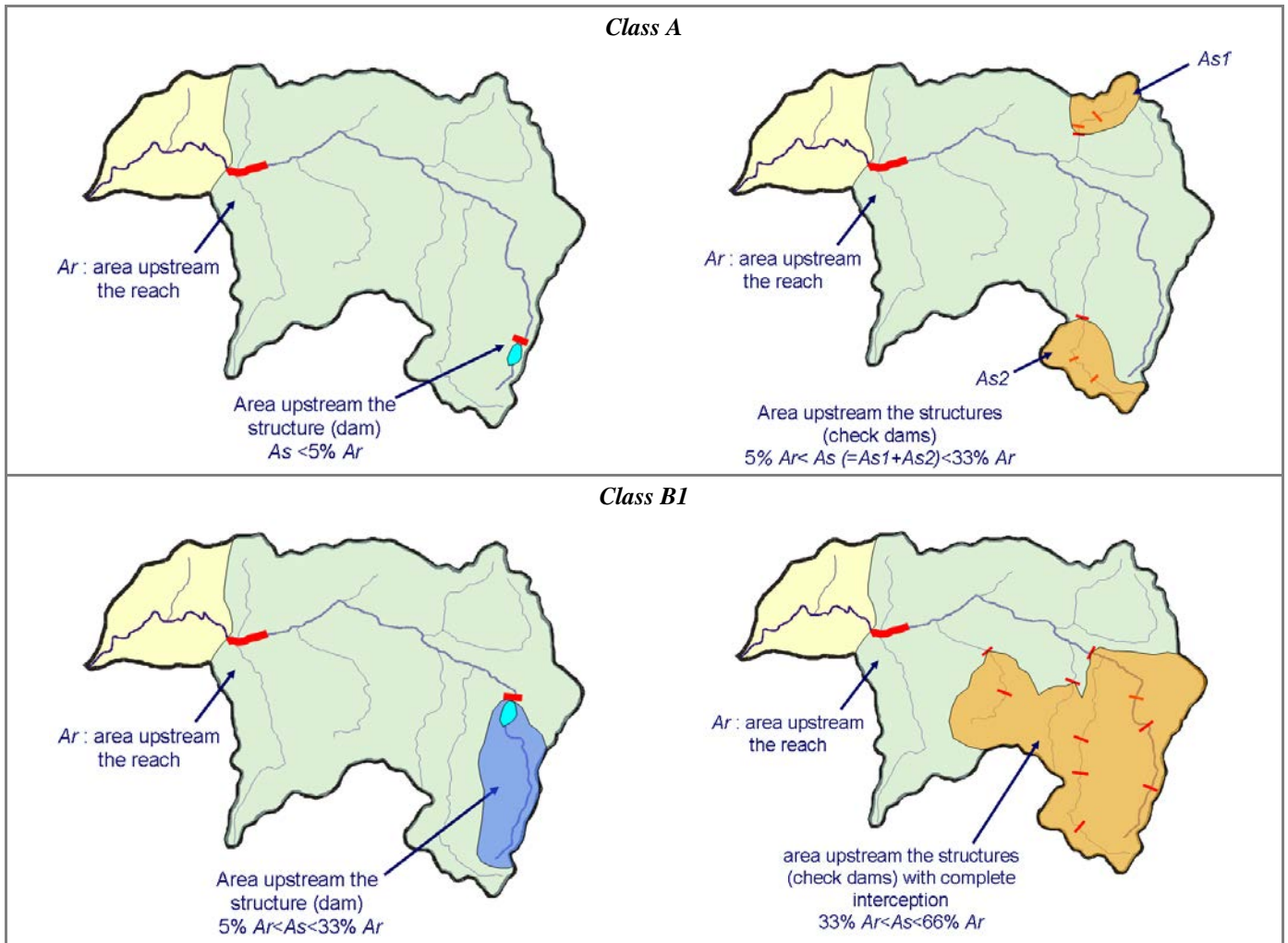
Figure 57 – Upstream alteration of sediment discharges. Class A : dam with a negligible drainage area ( < 5\% of the area upstream from the reach, A_r ) (left); the total area of portions of the watershed with check dams is < 33\% of the area upstream from the reach (right). Class B1 : dam with a drainage area between 5\% and 33\% of the area upstream from the reach (left); the total area of portions of the watershed with check dams is between 33\% and 66\% of the area upstream from the reach (it applies in the case of reaches in hilly or lowland areas) (right).
