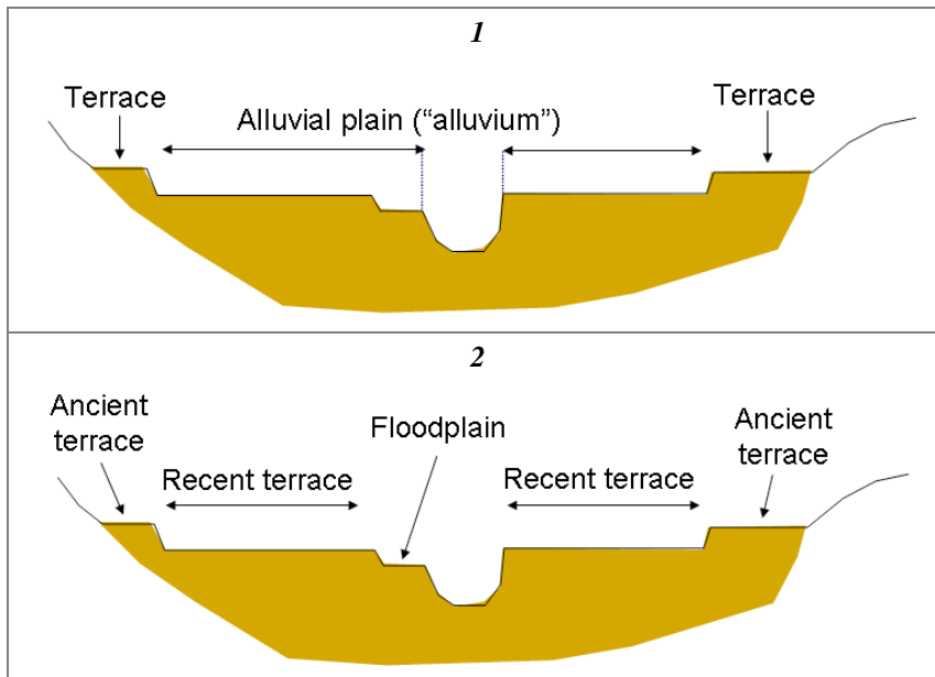
Figure 22 – Distinction between alluvial plain and floodplain. (1) Terminology commonly used on geological maps; (2) terminology adopted here (the alluvial plain can include both floodplain and “recent” terraces, which are previous portions of a floodplain abandoned due to incision during the last 100÷150 years).
