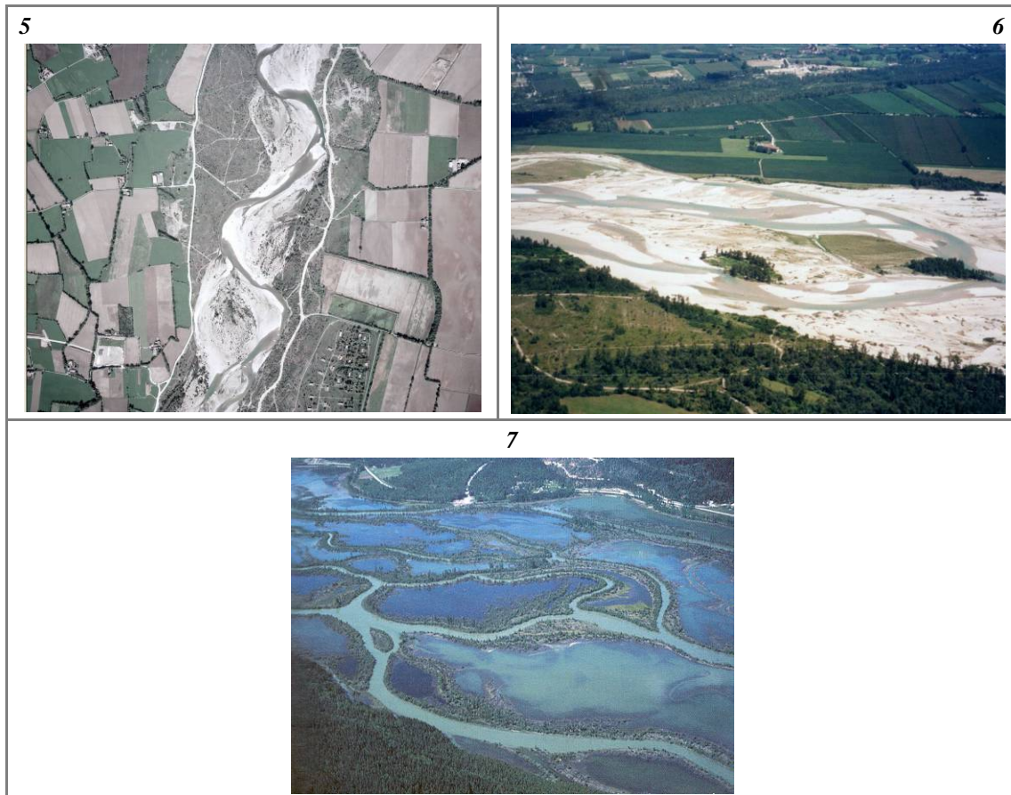
Figure 6 (continued) – Examples of morphologies of semiconfined and unconfined channels. (5) Wandering; (6) braided; (7) anastomosing (the islands and floodplain are inundated).
