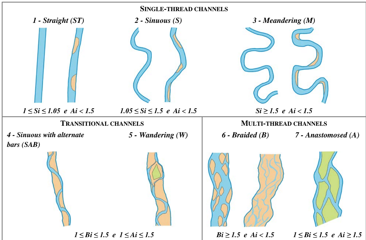
Figure 5 – Morphologies of semiconfined and unconfined channels. Si : sinuosity index; Bi : braiding index; Ai : anastomosing index.
