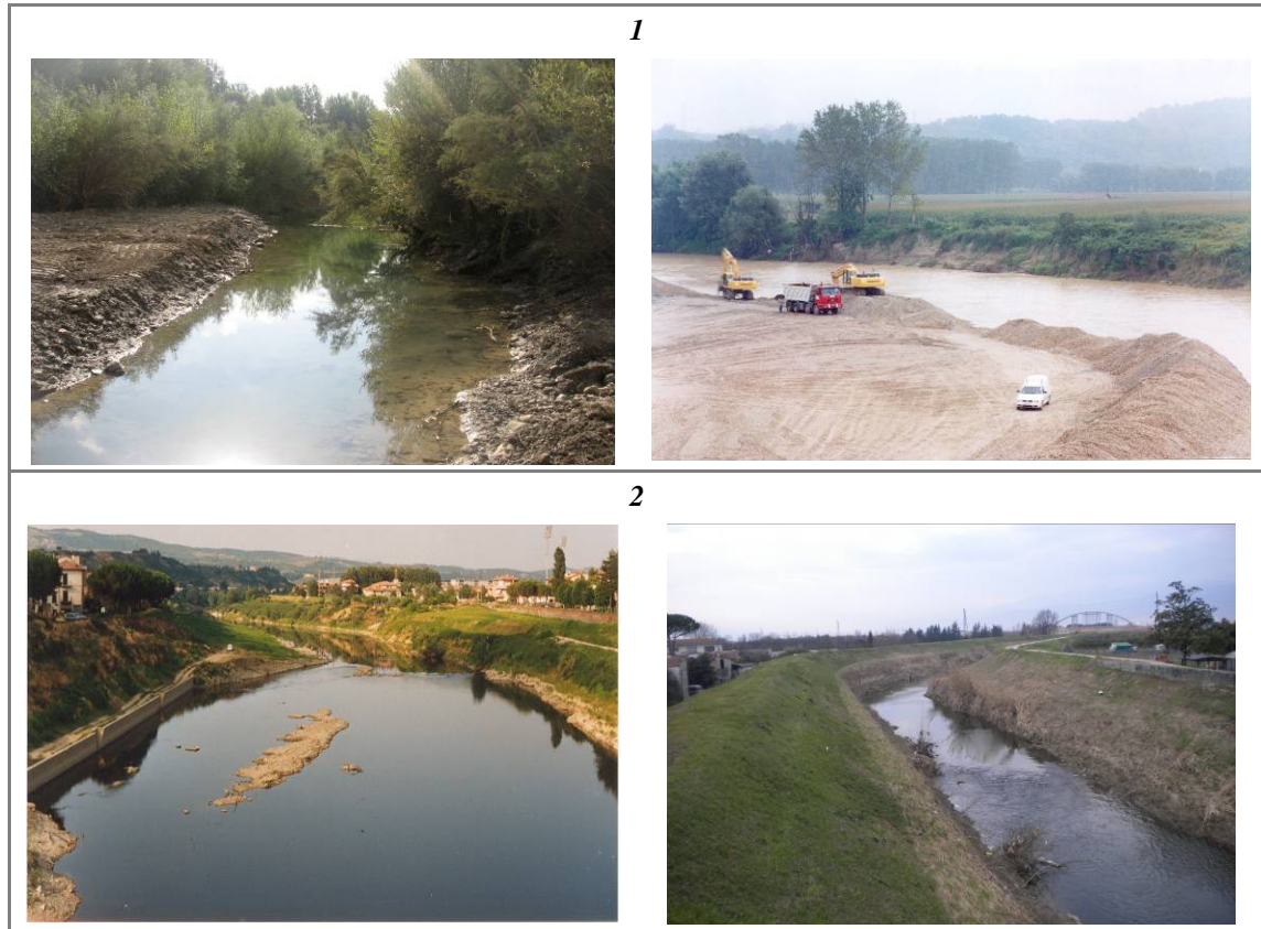
Figure 40 – Alteration of cross-section variability in semi- and unconfined channels. (1) Cases of partial homogenization of the cross-section due to interventions. (2) Cross-section homogeneity extended for long reaches due to excessive artificiality.
