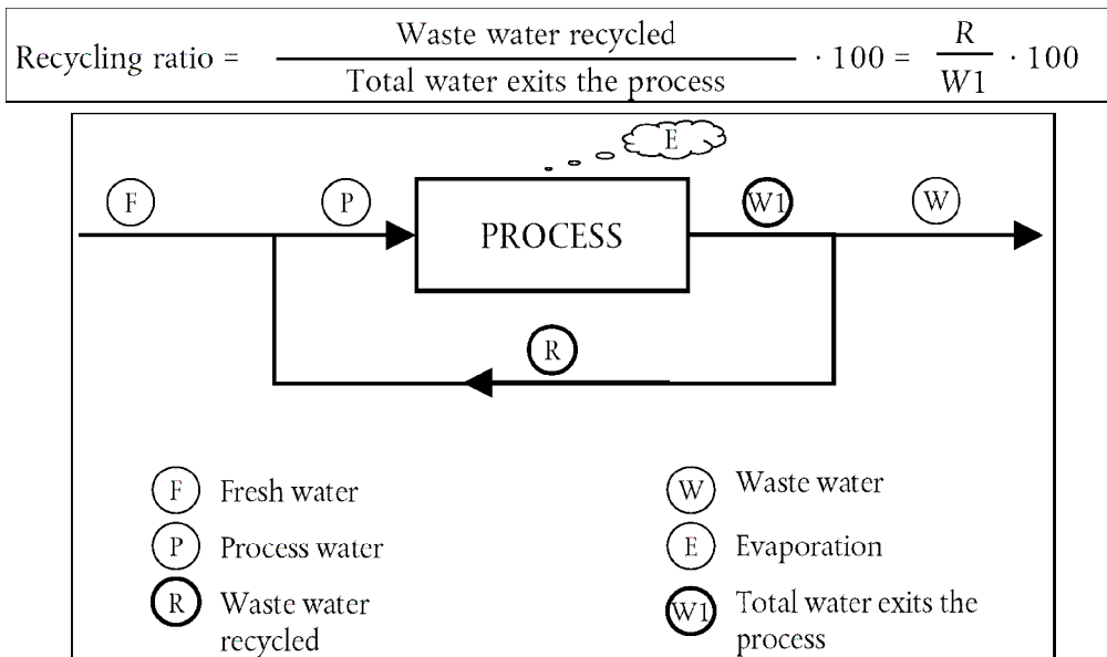
Figure A2: Water flow scheme that shall be used to calculate Water Recycling Ratio 10
