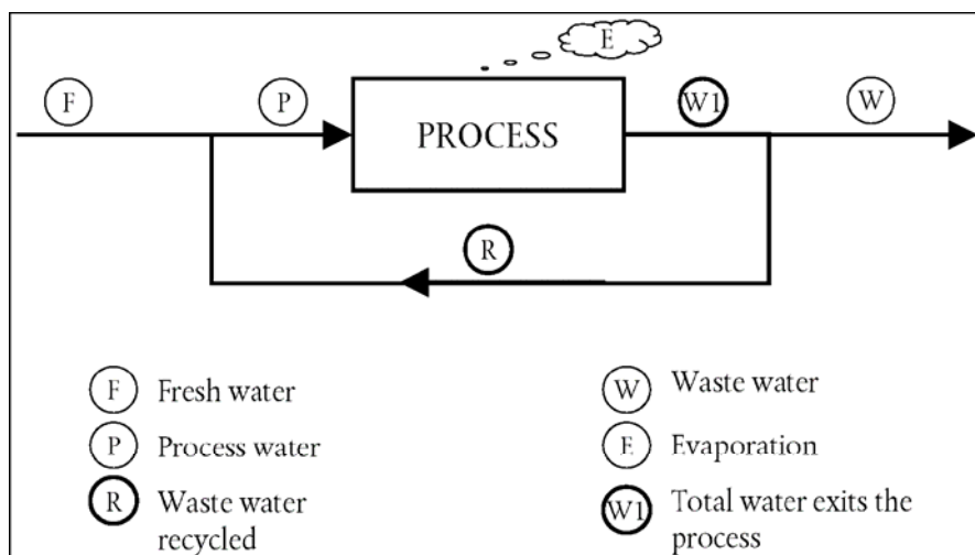
Figure A2: Water flow scheme that shall be used to calculate Water Recycling Ratio 12
