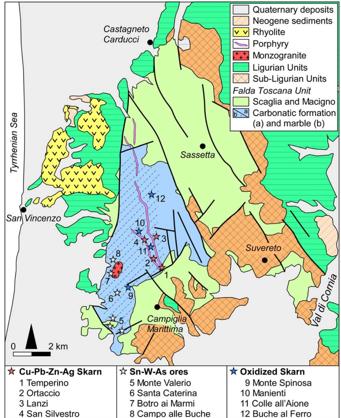
Fig. 6 - Geological sketch map of the Campigliese area showing the distribution of magmatic rocks and ore deposits (modified after Da Mommio et al., 2010).
