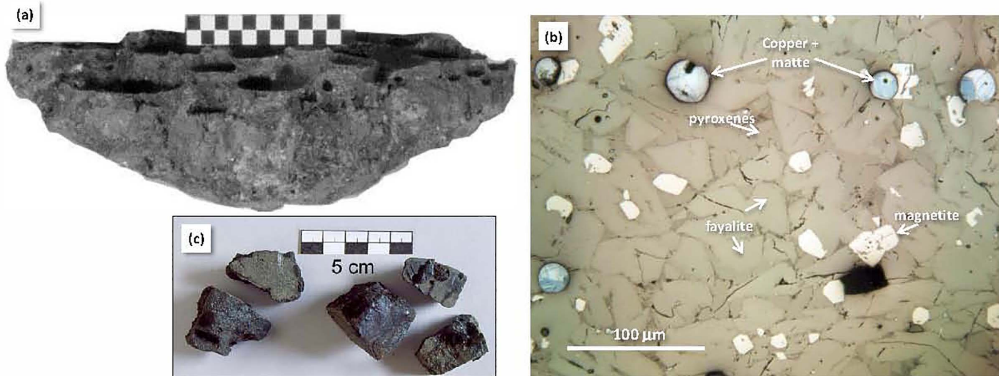
Fig. 43 – Macroscopic and microscopic features of copper slag from the Baratti beach slag deposit: (a) copper slag cake; (b) reflected light microscope image of a matte-rich copper slag showing several matte ( \pm copper) droplets in a matrix of fayalite, pyroxenes and subhedral magnetite crystals; (c) fragments of copper slag.
