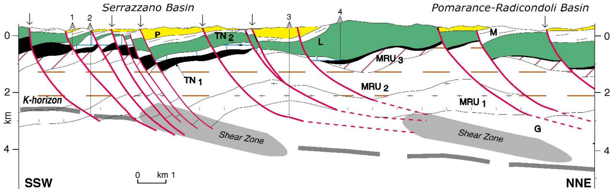
Fig. 24 - Geological section of the Larderello area obtained integrating borehole stratigraphies, field data, and reflection seismics interpretation. The K-horizon is interpreted as the upper boundary of an active shear zone (see text). Locations of outcropping normal faults are shown by black arrows. Key: P - Pliocene sediments; M - Miocene sediments; L: Ligurian and Sub-Ligurian complex; Tuscan nappe (TN): TN 2 - Early Miocene - Rhetic sequence; TN 1 - Late Triassic evaporites; Monticiano - Roccastrada unit (MRU): MRU 3 - Mesozoic - Paleozoic group; MRU 2 - phyllite - quartzitic group; MRU 1 - Paleozoic micaschist group; G: gneiss complex. Modified from Brogi et al. (2003).
