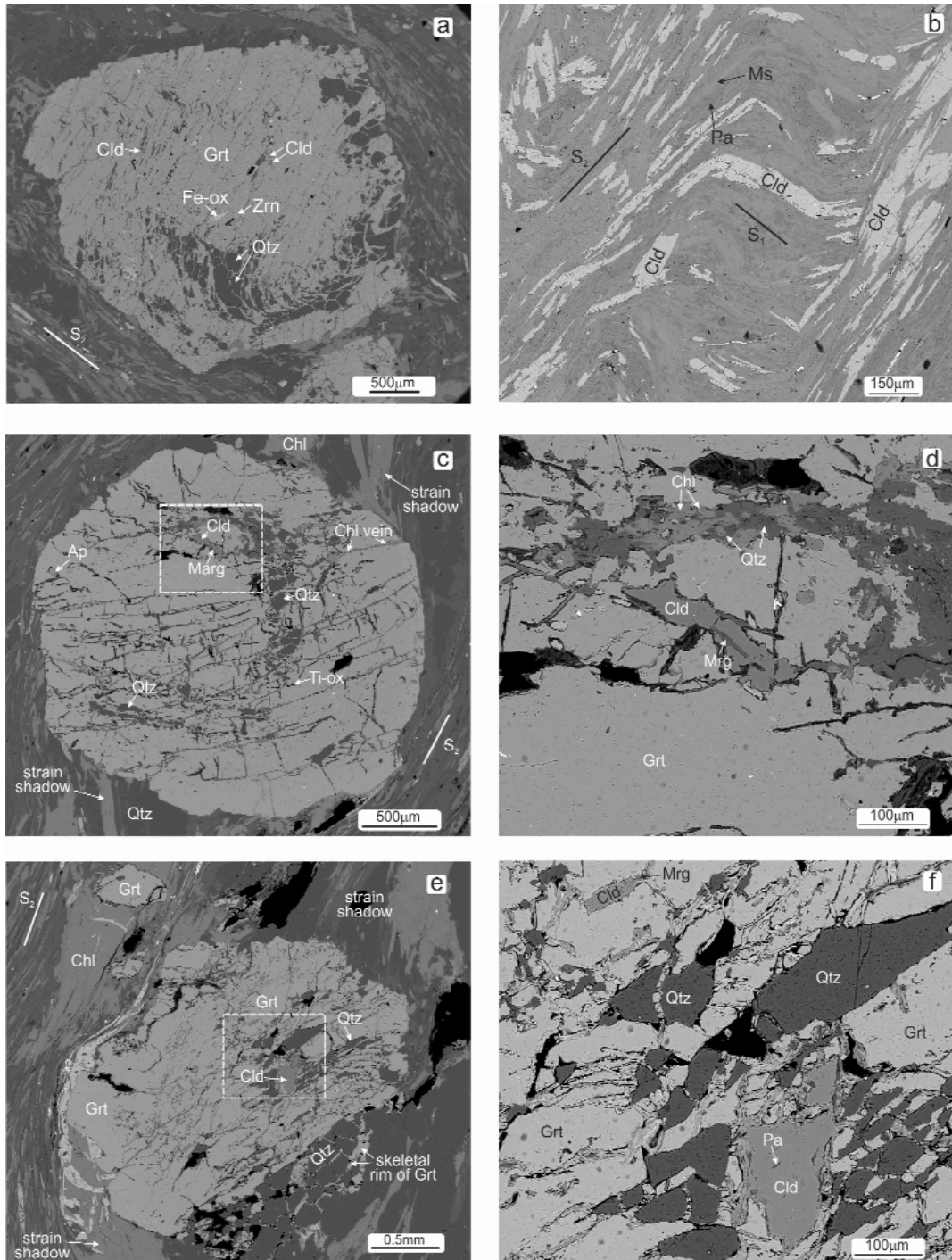
Fig. 1.11 - SEM images showing microstructural features of the chloritoid schists: a) inclusions in garnet; b) relationships between minerals and foliations; c) garnet with inclusions and strain shadows; d) margarite growth on chloritoid included in garnet; e) garnet with strain shadows of chlorite and skeletal quartz at garnet boundary; f) quartz and chloritoid inclusions in garnet (from Cruciani et al., 2013).
