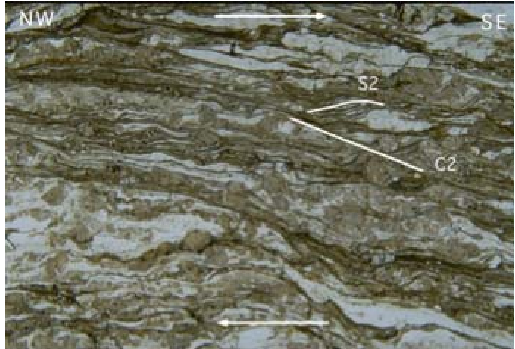
Fig. 1.25 - C-S fabric in mylonite from gneiss (PPL; fov is 7 mm).
