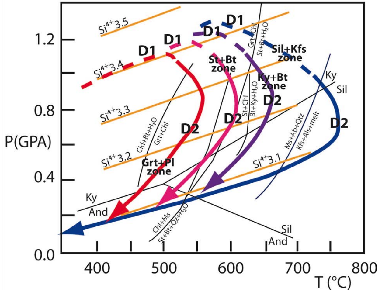
Fig. 6 - P-T-t paths for the various metamorphic zones of NE Sardinia (modified after Di Vincenzo et al., 2004).
