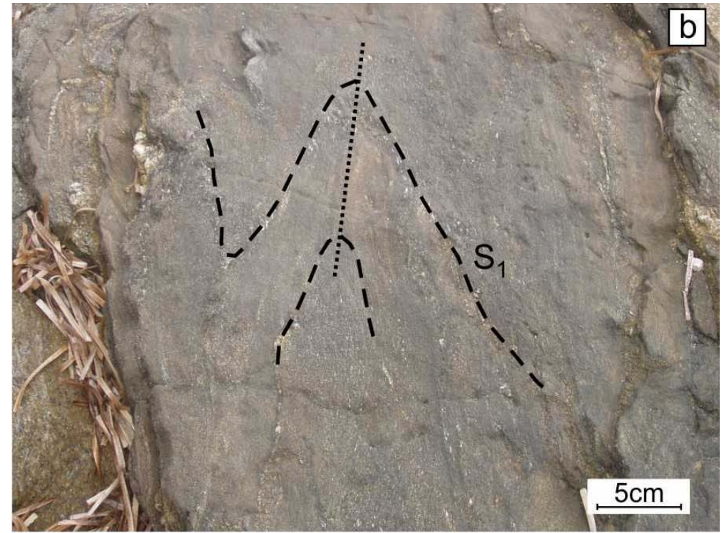
Fig. 2.13 - a) Contact between the migmatized orthogneiss (right) and the sedimentary-derived migmatite (left); b) intrafoliar D2 fold in the paragneiss of Porto Ottiolu with S2 axial plane schistosity which transposes an early S1 foliation.
