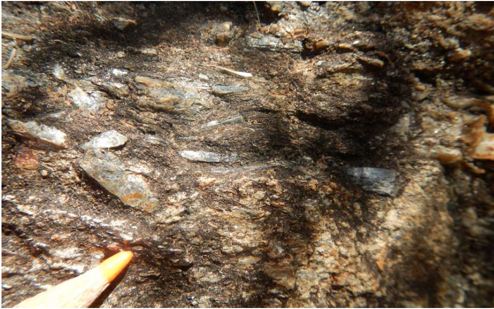
Fig. 2.5 - Mm to cm-size kyanite crystals aligned along the mylonitic foliation in the micaschist at Brunco Nieddu from the Ky + Bt zone.
