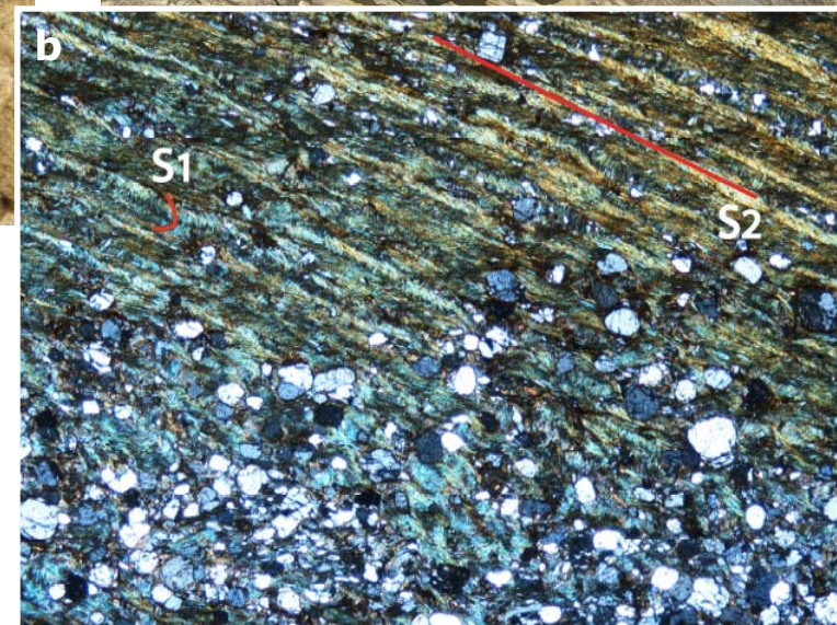
Fig. 1.5 - a) Albitic-rich layers in reworked metavulcanite folded by upright F2 folds. b) Photomicrograph showing the relationships between sedimentary bedding (sub-horizontal and marked by a change in composition of the layers), folded S1 foliation in the microlithons, and S2 crenulation cleavage axial plane of the metric F2 fold observed at the outcrop scale. The lower part is mainly composed of albite porphyroblasts. Crossed polars (CPL), 20x.
