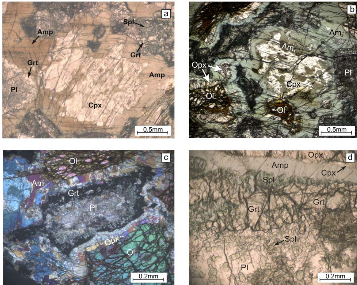
Fig. 3.17 - a) Magmatic clinopyroxene overgrown by brown amphibole; PPL; b) amphibole replacement of clinopyroxene in the rocks of Layer B of the ultramafic amphibolites; orthopyroxene around olivine can also be observed; PPL; c) garnet coronas around plagioclase at the interface between plagioclase and olivine in the rocks of Layer B; CPL; d) detail of corona between plagioclase and orthopyroxene; PPL, from Franceschelli et al. (2002).
