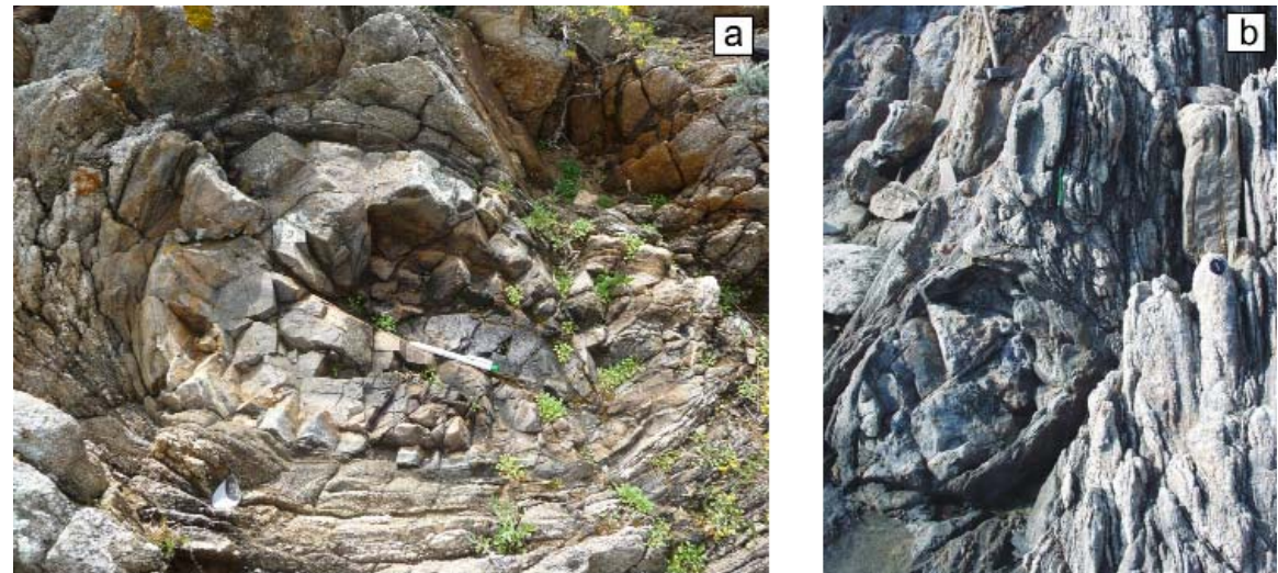
Fig. 3.13 - (a), (b) field appearance of calc-silicate nodules hosted in the Al-silicate-bearing migmatite outcrops north of Punta Sirenella.
