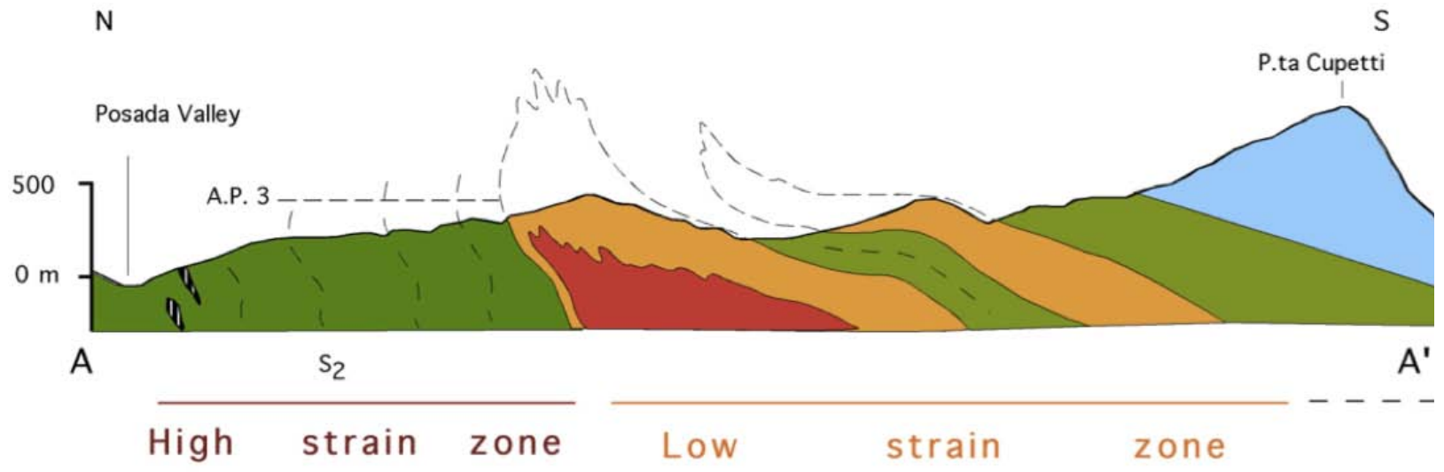
Fig. 1.18 - N-S geological cross section in the Posada Valley. See the geological map (Fig. 1.17) for explanations of the colours (modified after Carosi & Palmeri, 2002).
