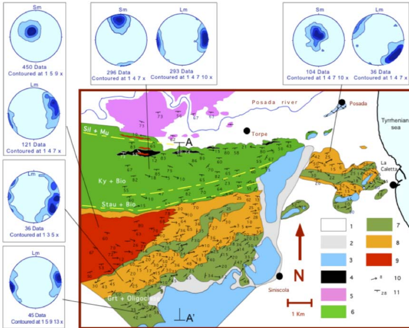
Fig. 1.17 - Geological and structural map of the Baronie area south of Posada Valley (modified after Carosi & Palmeri, 2002). 1 : Continental beach deposits (Pliocene-Quaternary); 2 : Slope debris (Quaternary); 3 : Carbonate platform sediments, continental and evaporites (Triassic - Jurassic - Cretaceous); 4 : Amphibolites with relics of granulite facies paragenesis; 5 : Migmatitic complex of Sil + Mu and Sil + K-feldspar zones (344+/-7 Ma); 6 : Micaschists and porphyroblastic paragneisses of St + Bt and Ky + Bt zones; 7 : Phyllites and metasandstones of Bt zone; micaschists and paragneisses of Grt + Ab and Grt + (Albite+Oligoclase) zones; 8 : Granitic augen gneisses (441+/-33Ma); 9 : Granodioritic orthogneisses (458+/-31 Ma); 10 : Trend and plunge of L2 stretching lineation; 11 : Strike and dip of mylonitic foliation (S2). A-A': trace of the geological cross-section of Fig. 1.18.
