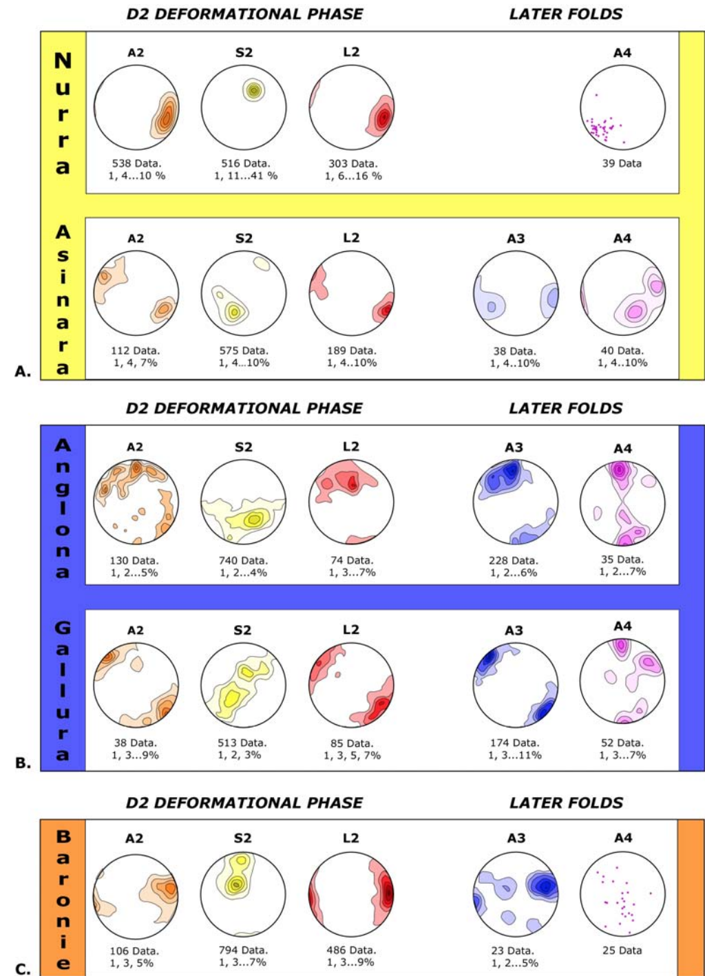
Fig. 5 - Stereographic projections (Schmidt equal area projection, lower hemisphere) of the main structural elements (D2-D4 deformation phases) in Northern Sardinia (from Carosi et al., 2005, 2006). A. Nurra-Asinara zone; B. Anglona-SW Gallura zones; C. Baronie zone. A2: axes of F2 folds; S2: second phase schistosity; L2: object and mineral lineation. A3 and A4 refer to later fold axes.
