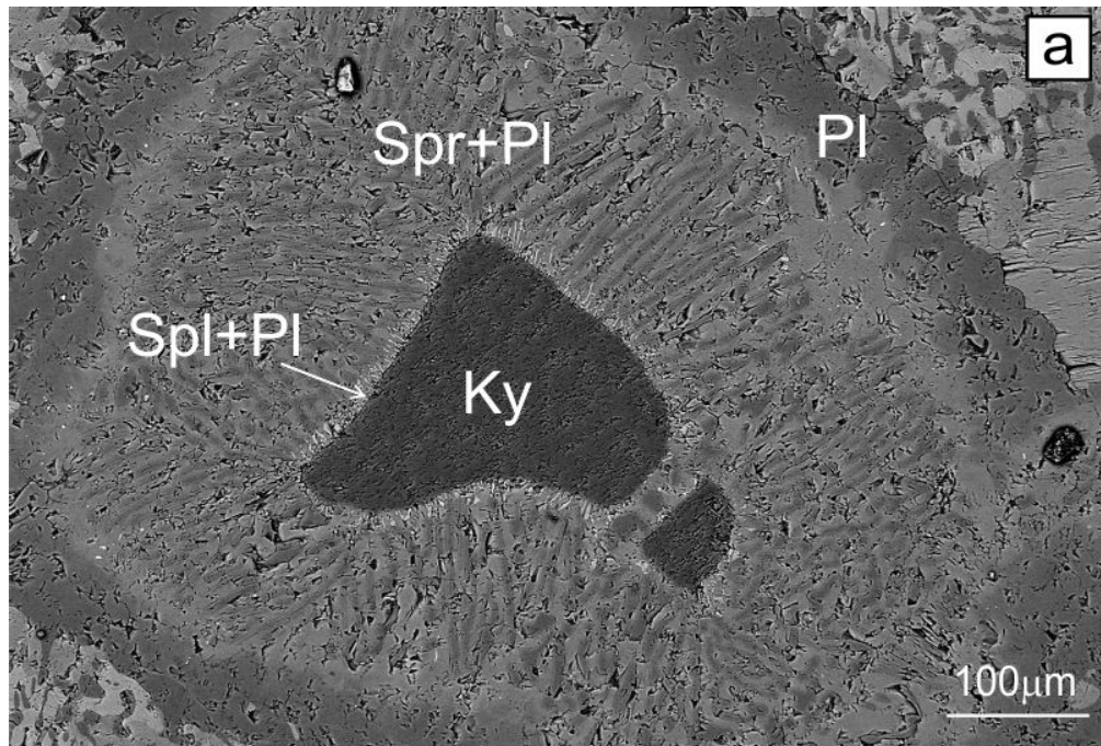
Fig. 3.21 - SEM images showing microstructural features of the retrogressed eclogite: a) kyanite surrounded by a thin layer of spinel + anorthite symplectite, in turn surrounded by a thicker layer of symplectitic plagioclase + sapphirine; b) corundum + plagioclase intergrowth.
