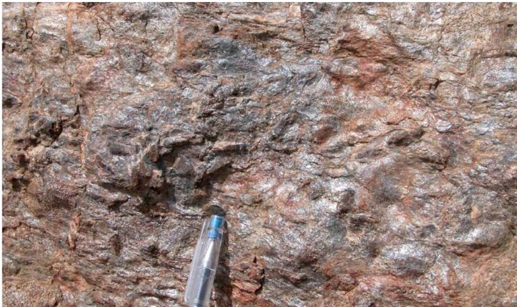
Fig. 2.3 - Cm-size staurolite porphyroclasts (brown-reddish crystals) developed on the S2 foliation in schists at the beginning of the road to Bruncu Nieddu St+Bt zone.
