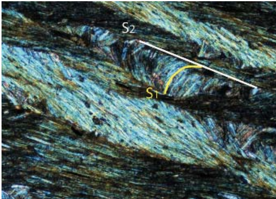
Fig. 1.6 - Detail of the relationship between S1 foliation in the microlithons and S2 crenulation cleavage in pelite-rich layers. (CPL), 60x.
