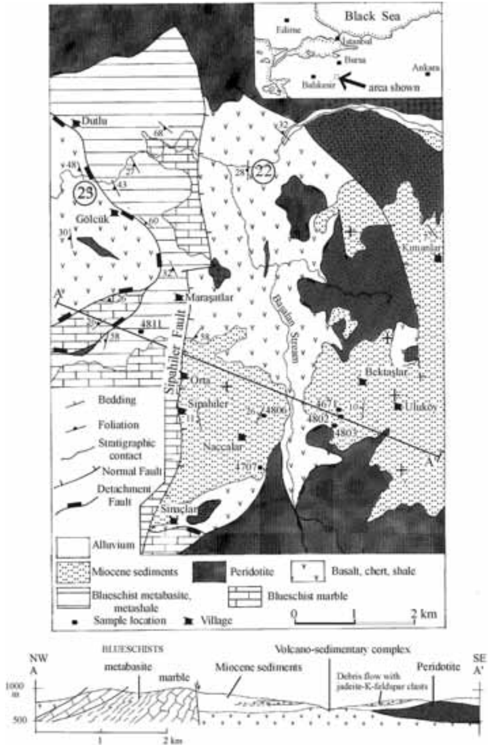
Figure 16 - Geological map and cross-section of the region west of Harmancik (after Okay, 1997).
