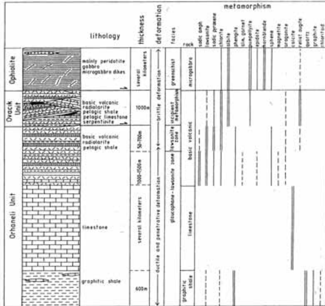
Figure 6 - Stratigraphy, lithology, structural features and mineral paragenesis of the Tavsanlı Zone (Okay, 1986).
