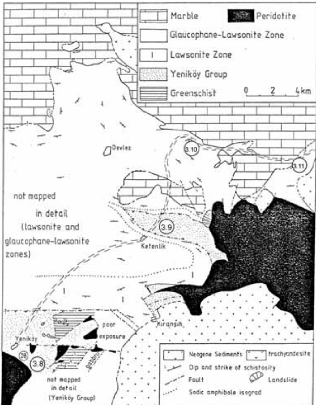
Figure 18 - Geological map of the region northeast of Tavşanlı showing the location of Stops 3.8 to 3.11. For location see Figure 5 (Okay, 1981).
