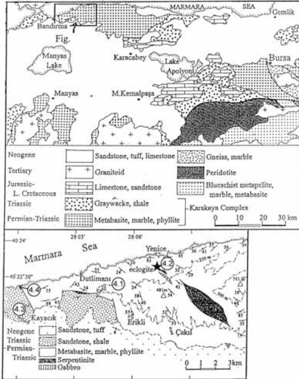
Figure 19 - Geological map of the region east of Bandırma showing Stopns 4.1 to 4.4. For location see Figure 3 (Okay and Monie 1997).
