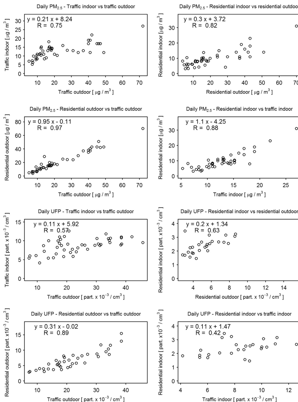
Fig. 2. Scatter plot for daily PM_{2.5} mass and UFP number.
