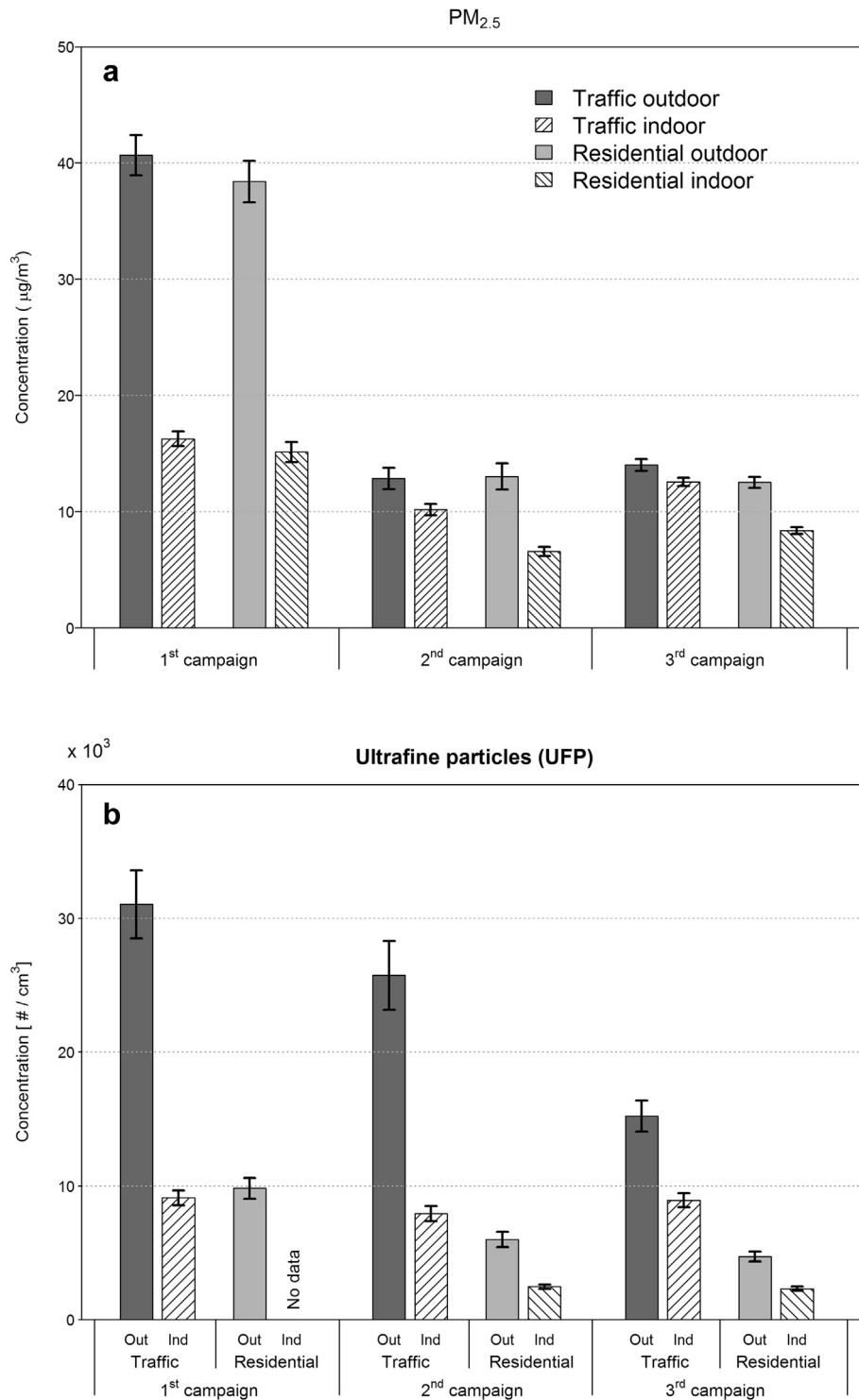
Fig. 1. Average value and standard error of PM 2.5 (a) and UFP (b) during the three monitoring campaign.
