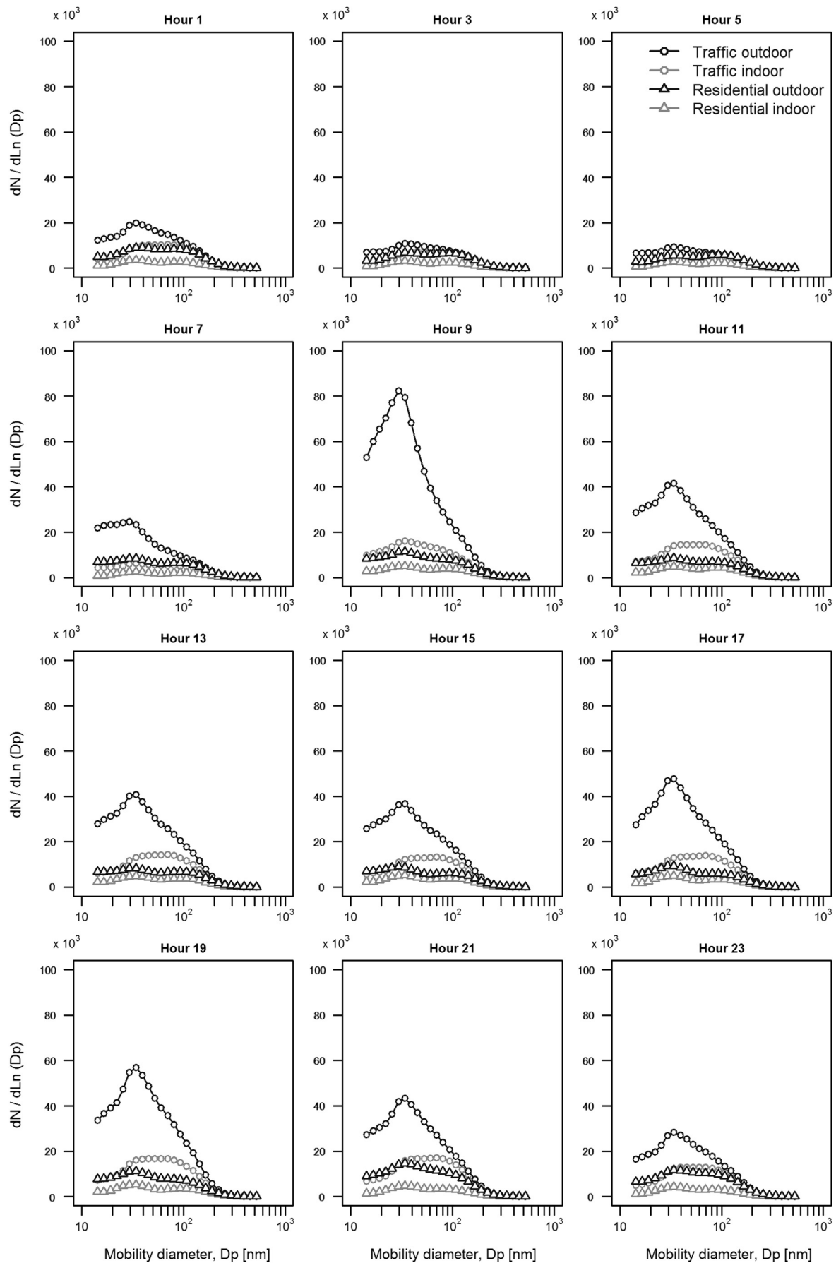
Fig. 7. Mean particle size distribution of hourly data at specific time of the day.
