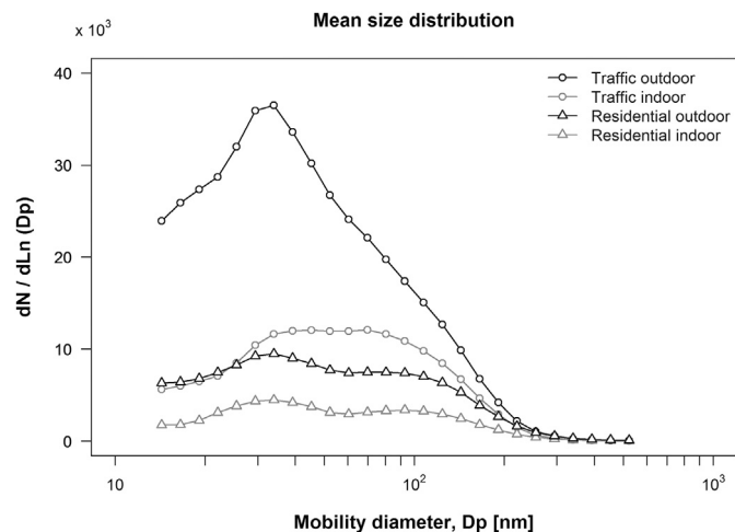
Fig. 6. Mean particle size distribution of hourly data.
