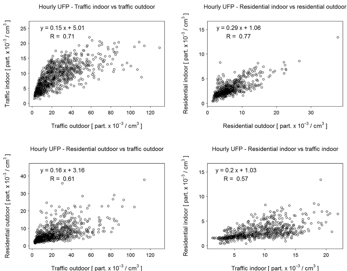
Fig. 4. Scatter plot for hourly UFP number.
