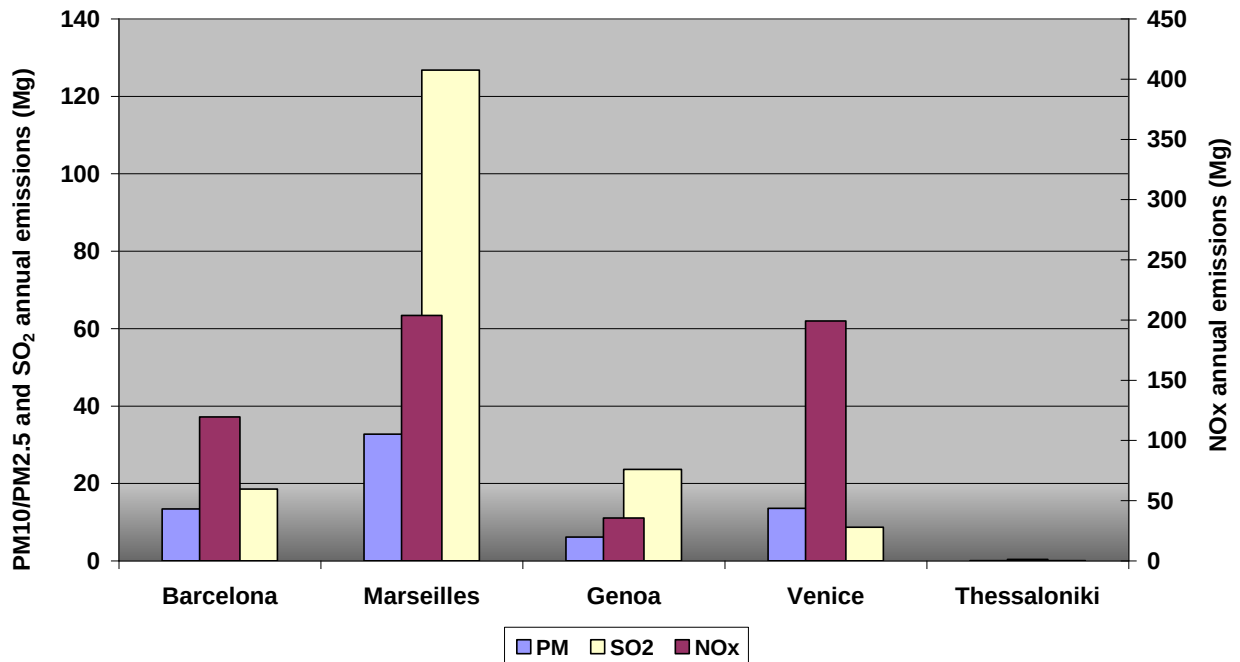
Fig. 1.3.1.4. Macropollutant emissions by cruise ships in maneuvering phase in 2013.
