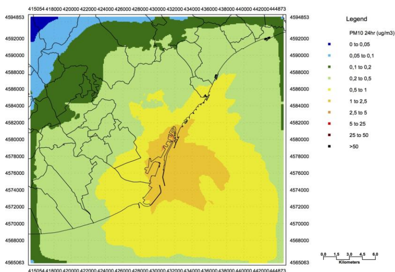
Fig. 2.2.1.2. 90.4% percentile of the 365 daily PM 10 concentrations. Reference year 2013.
