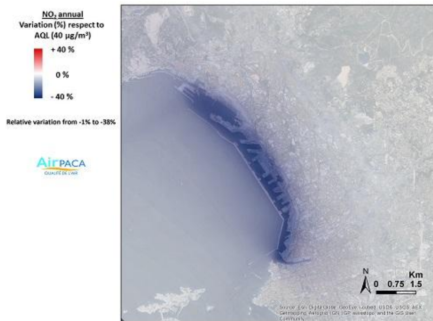
Fig. 5.2.3.1. Percentage differences in the NO 2 annual mean between LNG mitigation and future trend scenarios with respect to the corresponding AQL.
