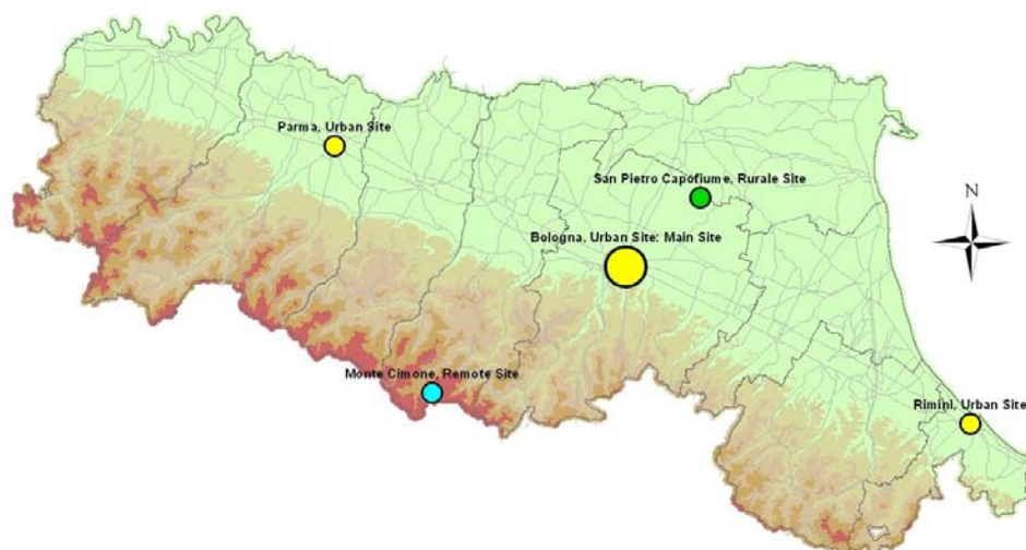
Fig. 1 – Sampling sites: Bologna (main site, MS), Parma (US1), Rimini (US2), San Pietro Capofiume (RS3) and Monte Cimone (RS4).
