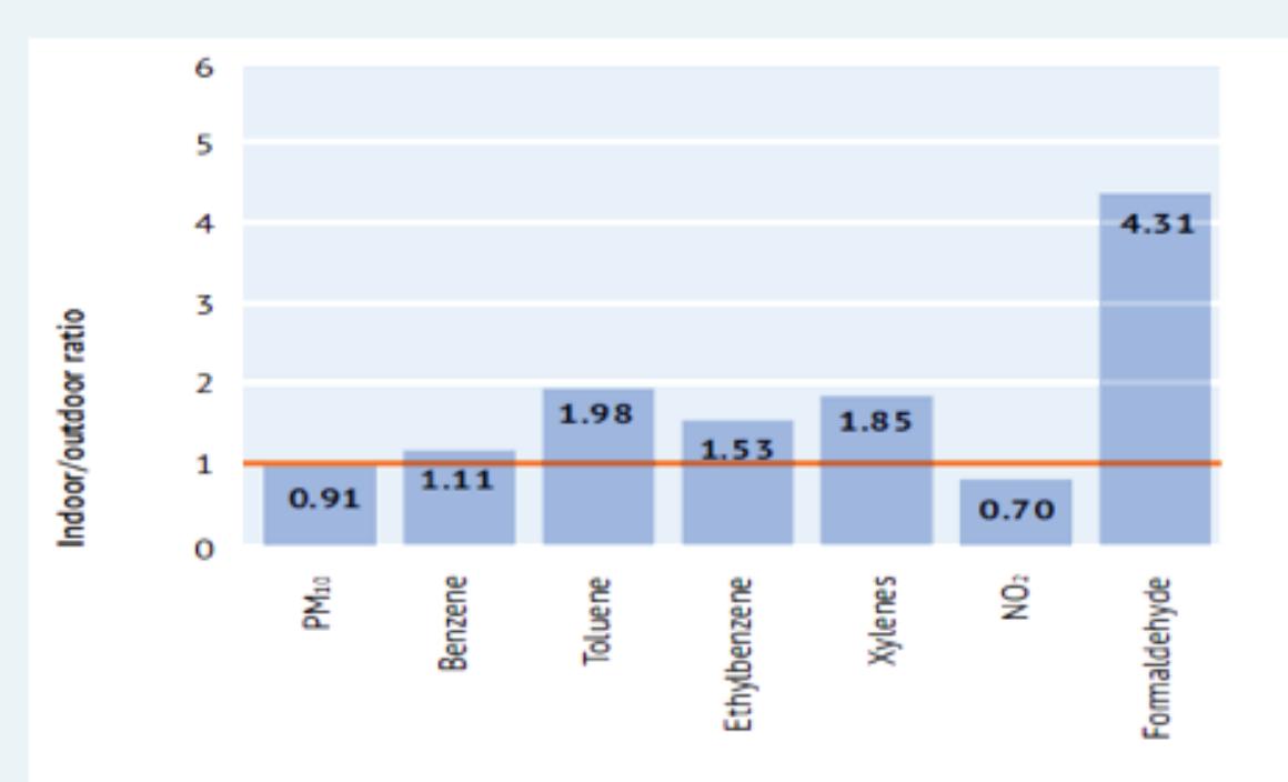
Relationship between concentrations measured inside the classrooms and outside the schools in the 10 SEARCH countries
