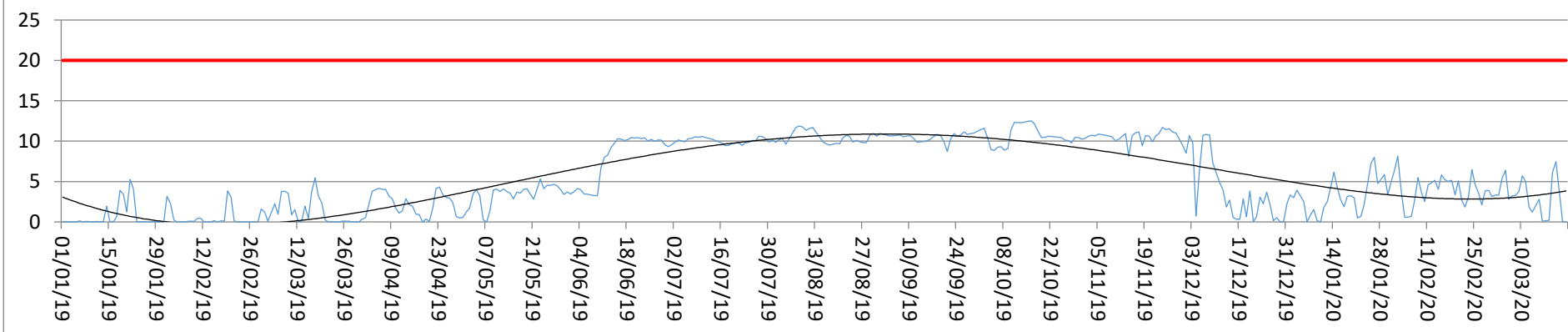
SOx (mg/Nm3) camino E525B - Anni 2019-2020
