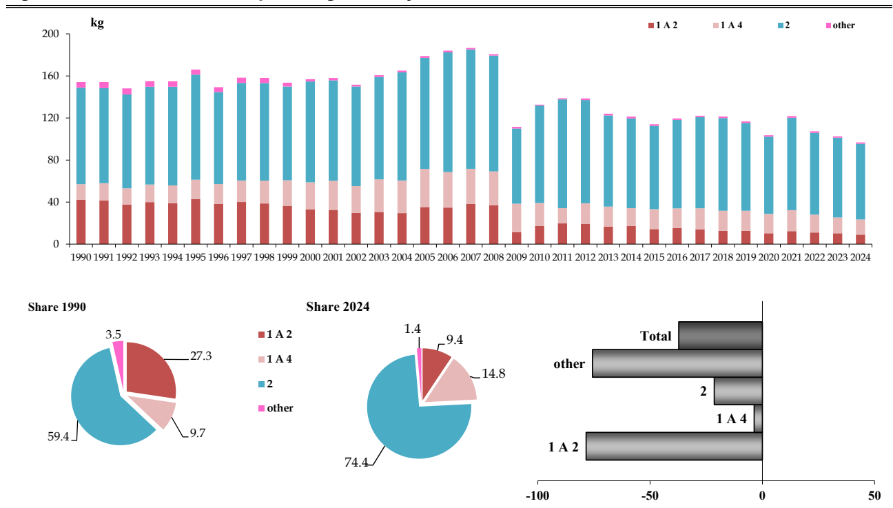
Figure 2.15 PCB emission trend, percentage share by sector and variation 1990-2024
