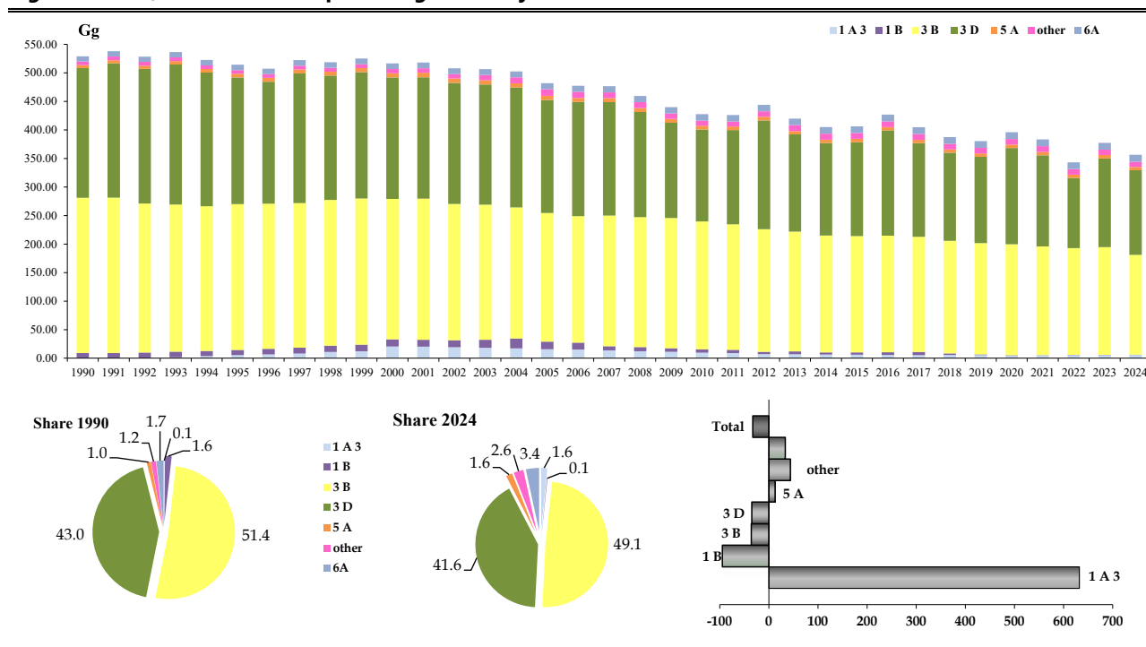
Figure 2.3 NH 3 emission trend, percentage share by sector and variation 1990-2024
