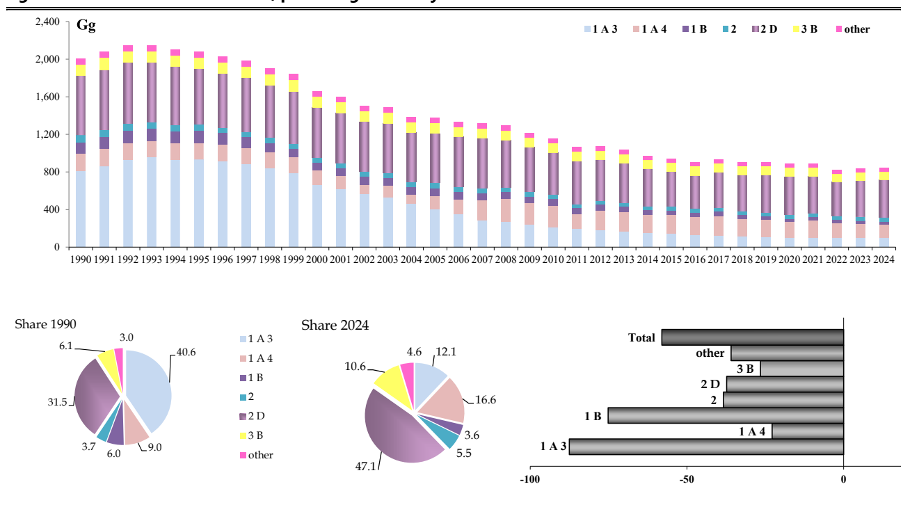
Figure 2.4 NMVOC emission trend, percentage share by sector and variation 1990-2024
