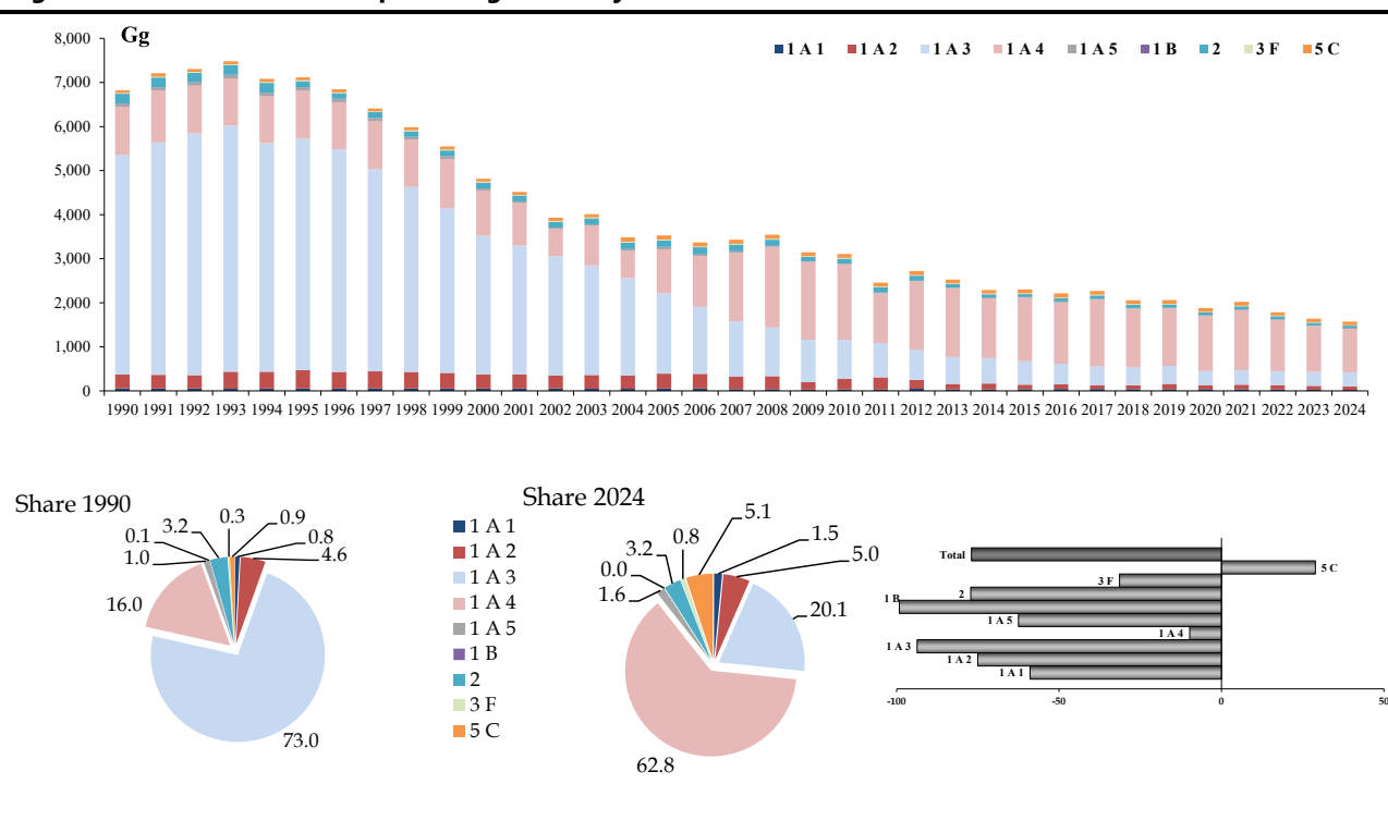
Figure 2.5 CO emission trend, percentage share by sector and variation 1990-2024
