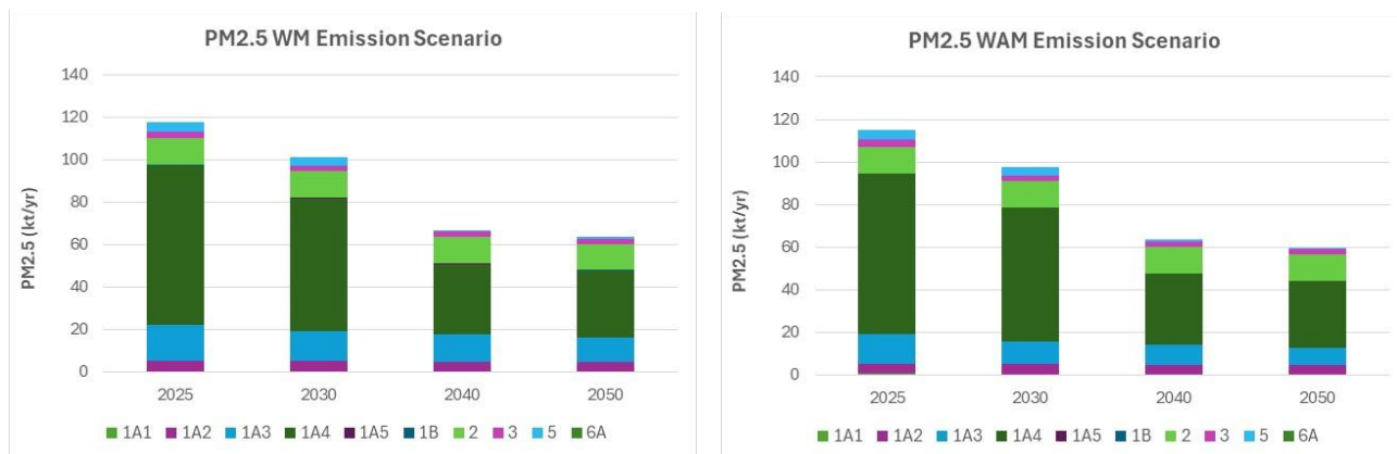
Figure 10.14 PM2.5 emission scenario WM (on the left) and WAM (on the right) by sector
