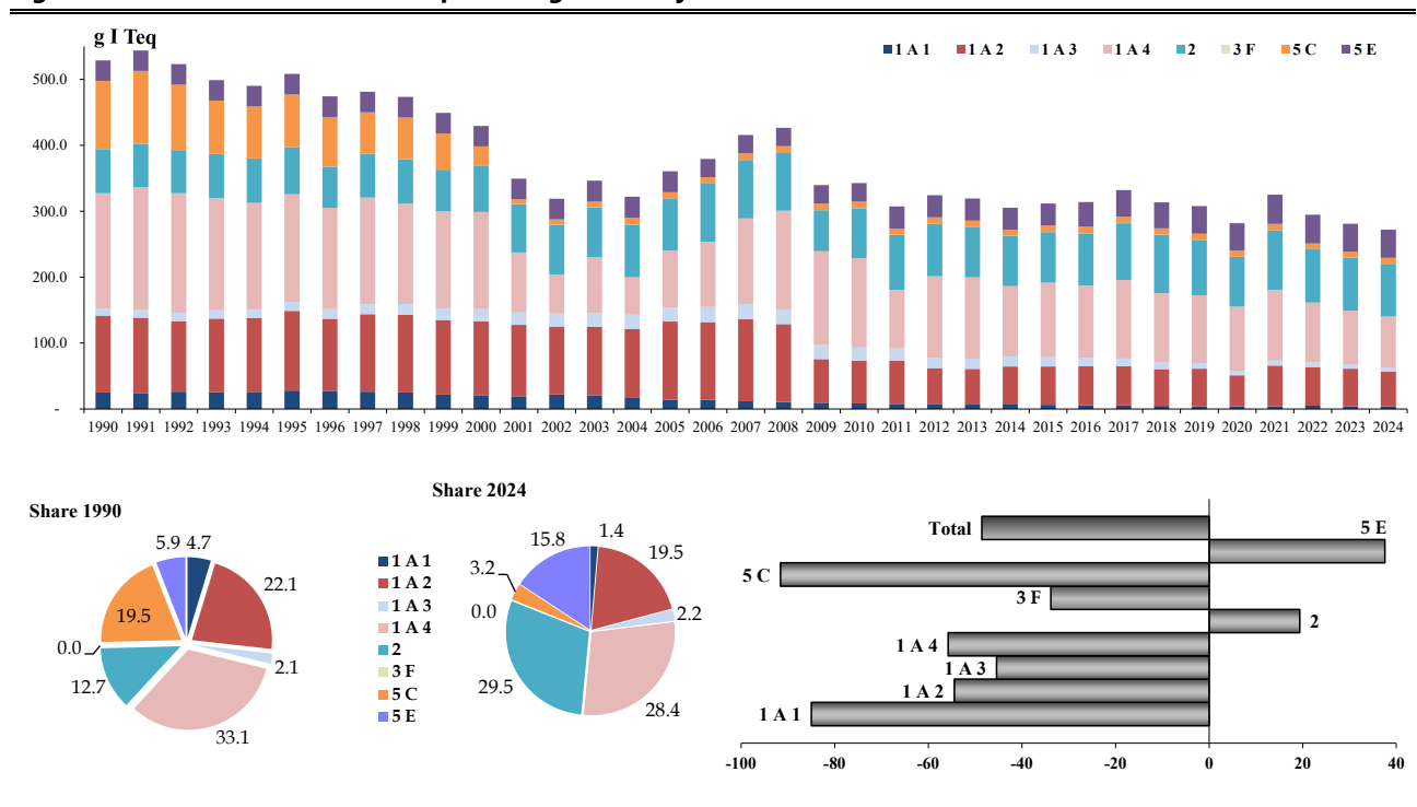
Figure 2.13 Dioxin emission trend, percentage share by sector and variation 1990-2024
