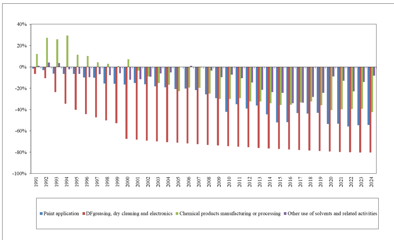
Figure 5.2 Trend of NMVOC emissions from 1991 to 2024 as compared to 1990
