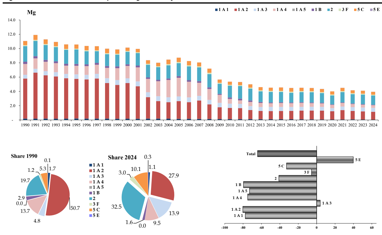
Figure 2.10 Cd emission trend, percentage share by sector and variation 1990-2024
