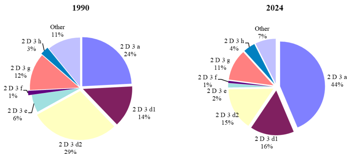
Figure 5.1 Share of NMVOC emissions for the solvent use sector in 1990 and 2024
