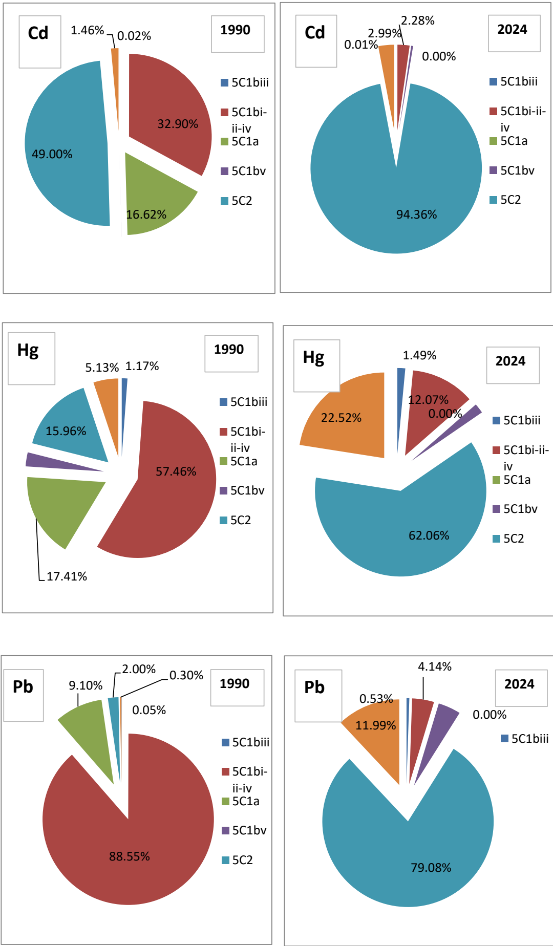
Figure 7.4 Contribution of priority heavy metals sub-category emissions to waste sector total emissions
