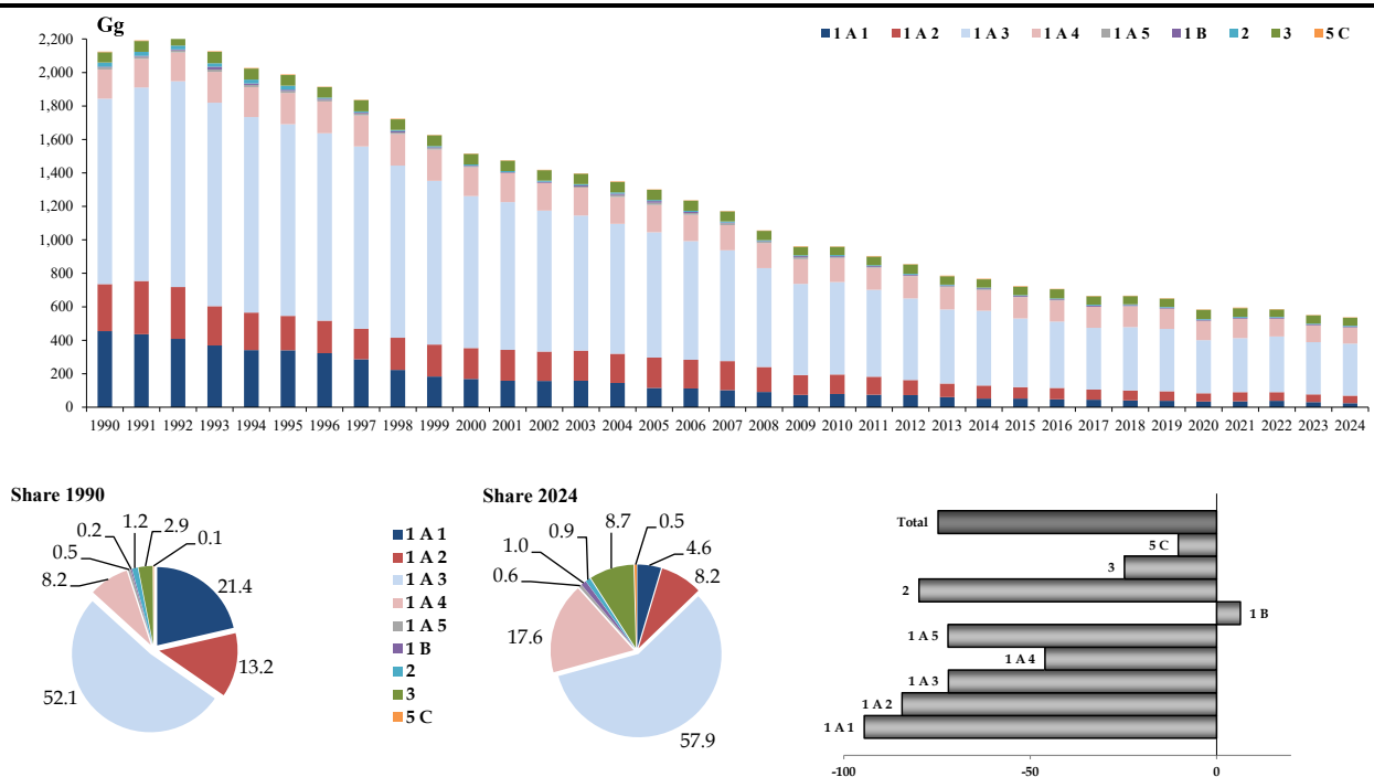
Figure 2.2 NO x emission trend, percentage share by sector and variation 1990-2024
