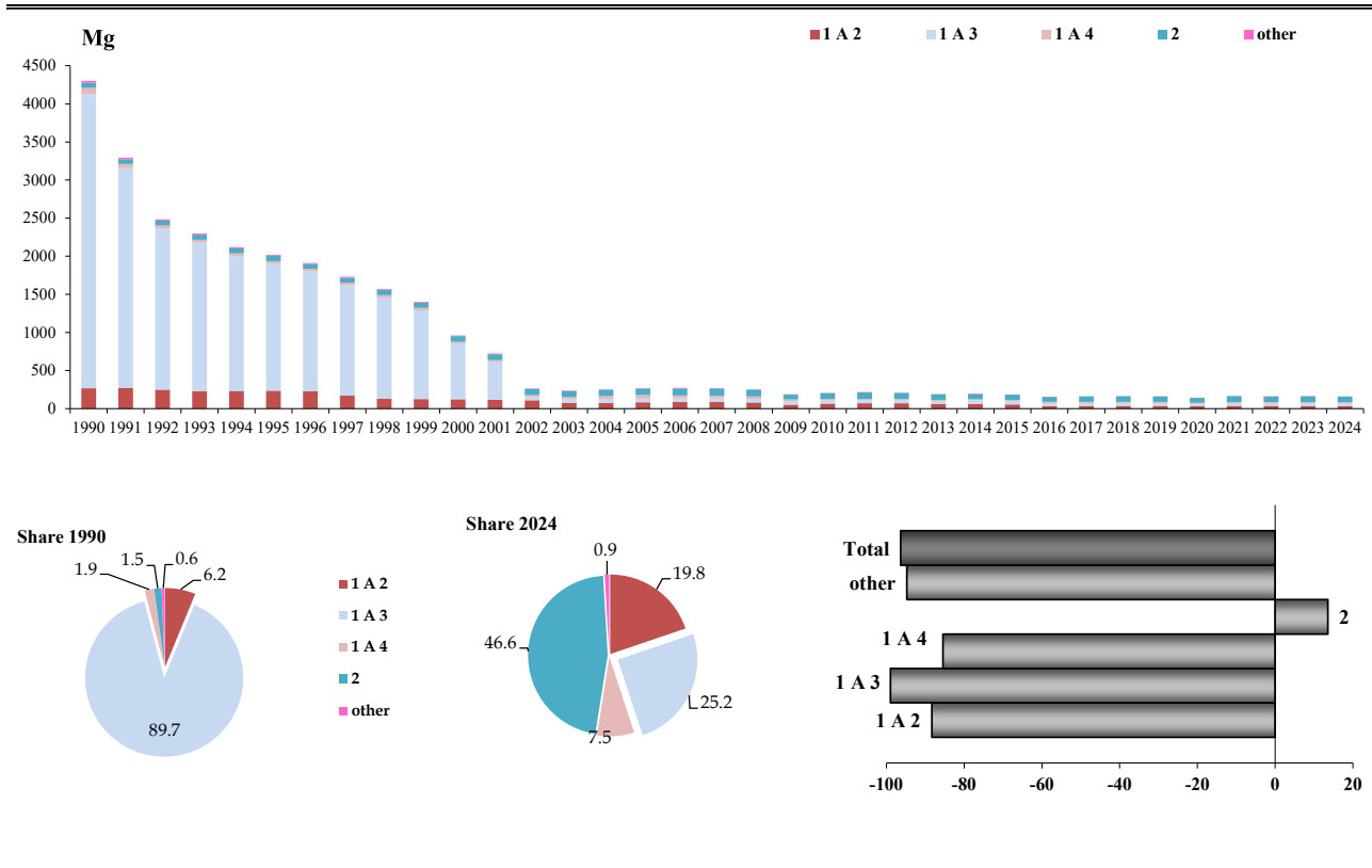
Figure 2.9 Pb emission trend, percentage share by sector and variation 1990-2024
