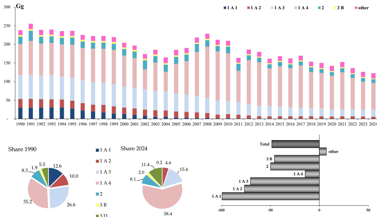
Figure 2.7 PM2.5 emission trend, percentage share by sector and variation 1990-2024
