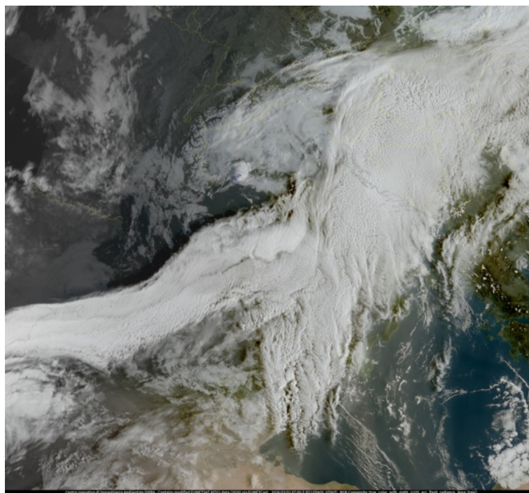
Figura 2: EUMETCast Meteosat-12 FCI Truecolor/10.5 \mu m + LI AFR 02/03/2026 ore 07:00 UTC
