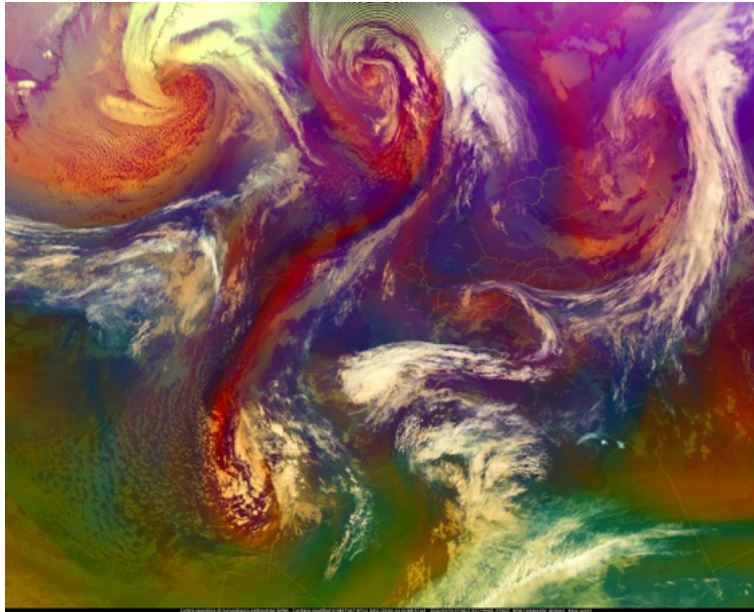
Figura 1: Meteosat-12 FCI FDHSI airmass 03/03/2026 ore 07:00 UTC
