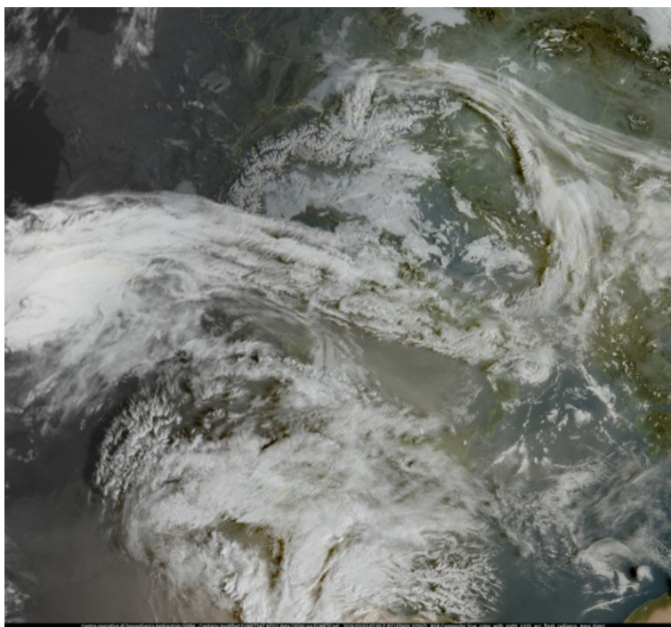
Figura 2: EUMETCast Meteosat-12 FCI Truecolor/10.5 \mu m + LI AFR 03/03/2026 ore 07:00 UTC
