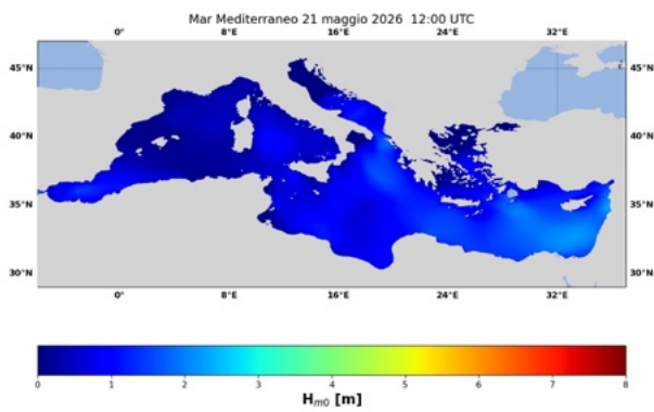
(a) ore 12 UTC 21/05/2026
