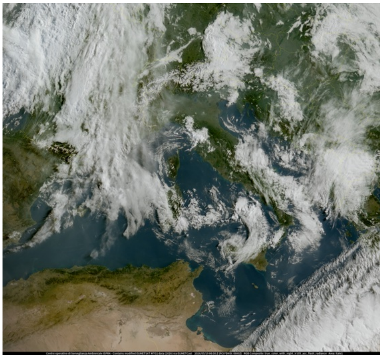
Figura 2: EUMETCast Meteosat-12 FCI Truecolor/10.5 \mu m + LI AFR 19/05/2026 ore 06:00 UTC
