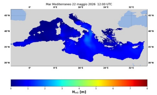
(b) ore 12 UTC 22/05/2026
