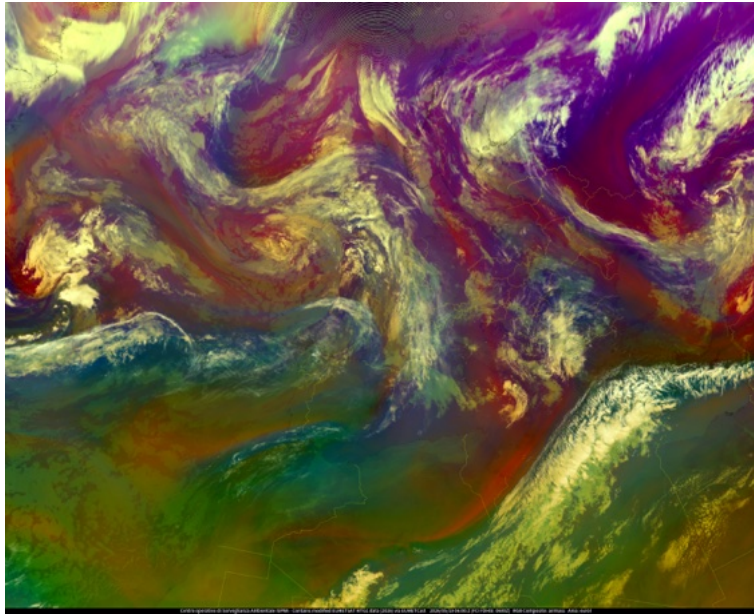
Figura 1: Meteosat-12 FCI FDHSI airmass 19/05/2026 ore 06:00 UTC
