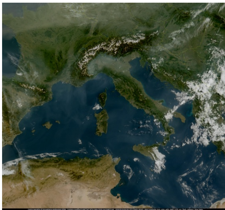
Figura 2: EUMETCast MTG FCI FDHSI IR 10.5/Truecolor+LI AFR 24/05/2026 ore 06:30 UTC.
