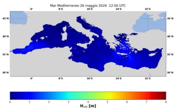
(a) ore 12 UTC 26/05/2026
