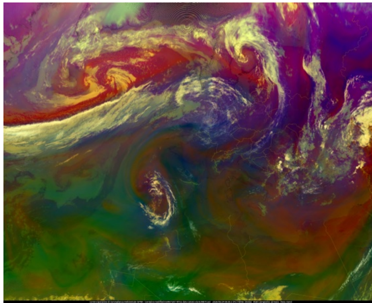
Figura 1: EUMETCast MTG FCI FDHSI airmass 24/05/2026 ore 06:30 UTC.
