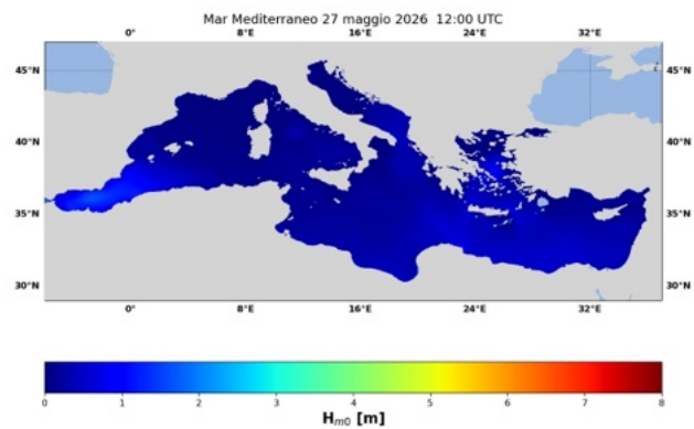
(b) ore 12 UTC 27/05/2026
