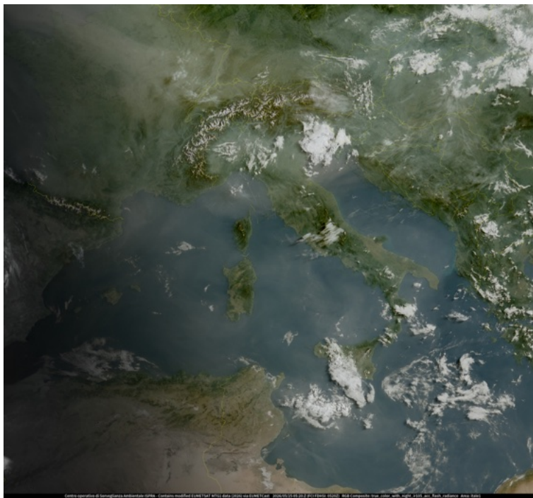
Figura 2: EUMETCast Meteosat-12 FCI Truecolor/10.5 \mu m + LI AFR 25/05/2026 ore 05:20 UTC
