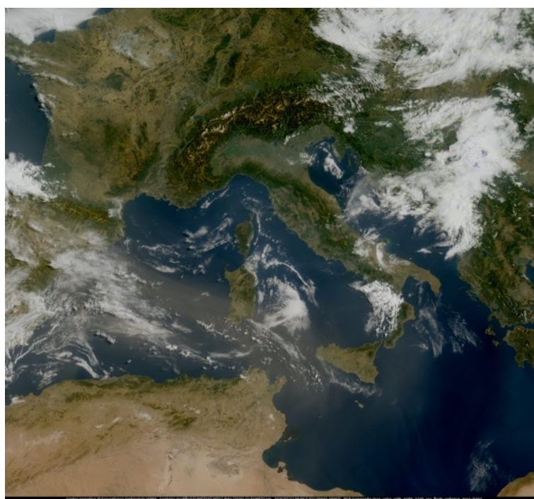
Figura 2: EUMETCast MTG FCI FDHSI IR 10.5/Truecolor+LI AFR 12/07/2026 ore 08:00 UTC.
