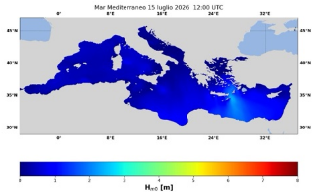
(b) ore 12 UTC 15/07/2026
