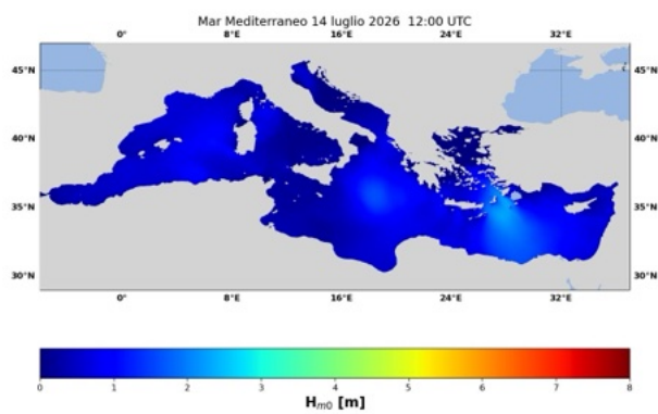
(a) ore 12 UTC 14/07/2026
