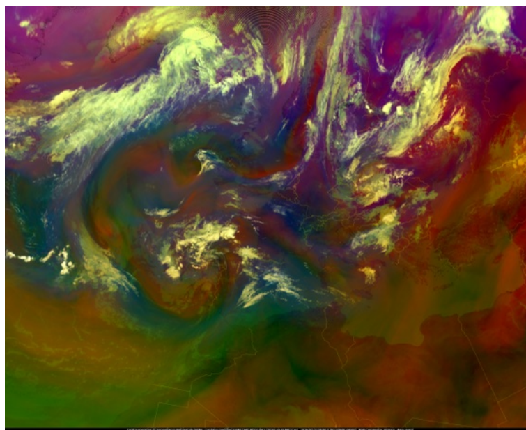
Figura 1: EUMETCast MTG FCI FDHSI airmass 12/07/2026 ore 08:00 UTC.
