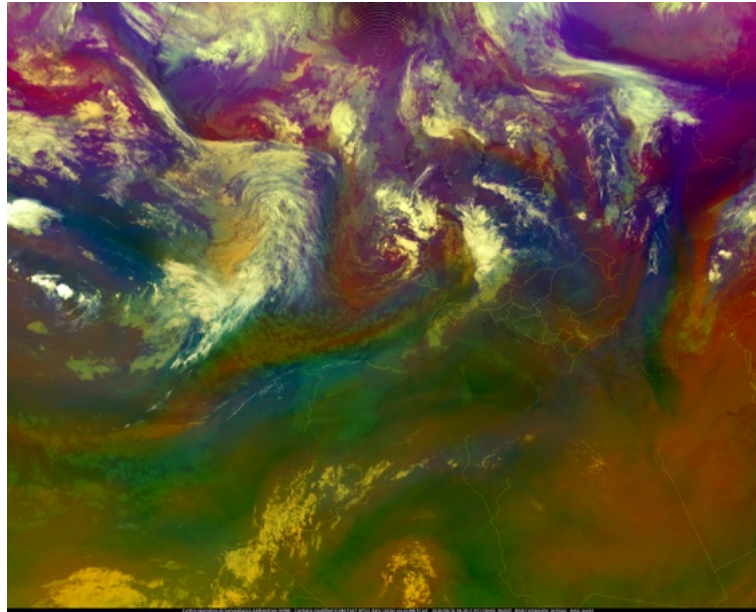
Figura 1: Meteosat-12 FCI FDHSI airmass 31/08/2026 ore 06:20 UTC
