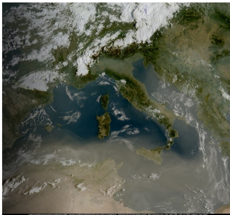
Figura 2: EUMETCast Meteosat-12 FCI Truecolor/ 10.5\mu\text{m} + LI AFR 31/08/2026 ore 06:20 UTC
