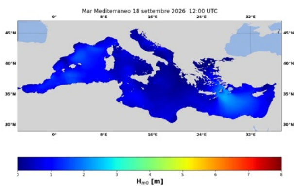
(a) ore 12 UTC 18/09/2026
