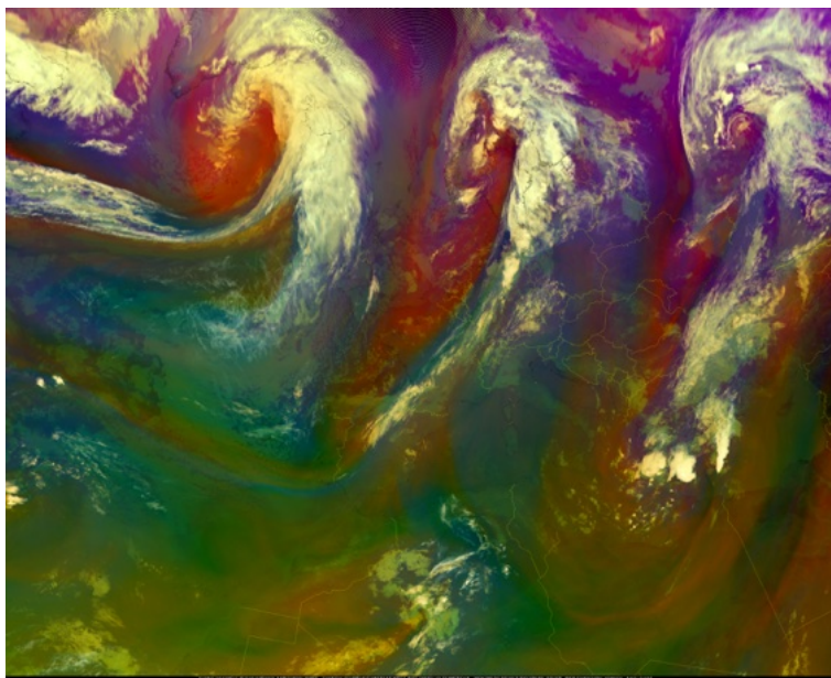
Figura 1: Meteosat-12 FCI FDHSI airmass 16/09/2026 ore 07:10 UTC
