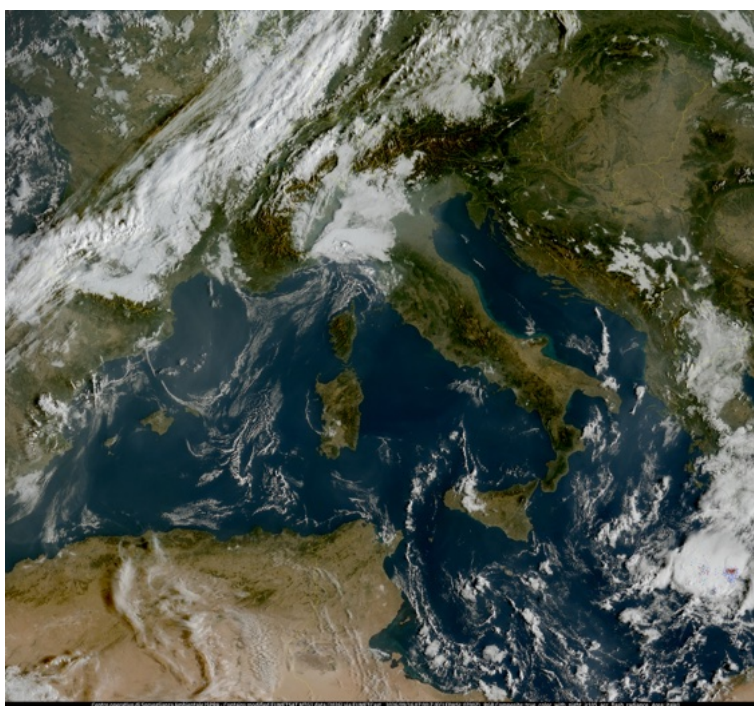
Figura 2: EUMETCast Meteosat-12 FCI Truecolor/ 10.5\mu\text{m} + LI AFR 16/09/2026 ore 07:00 UTC
