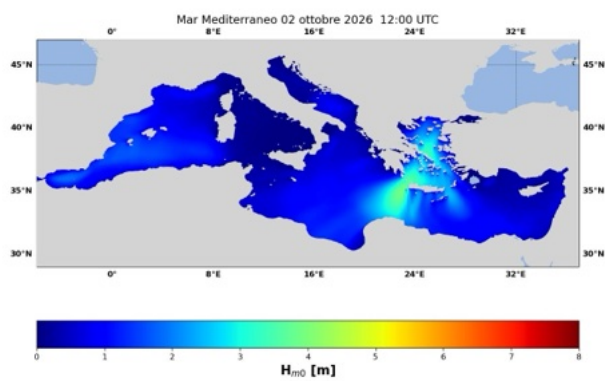
(a) ore 12 UTC 2/10/2026
