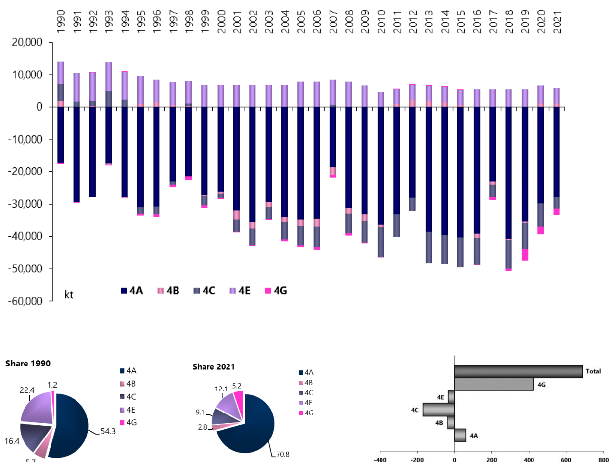
Figure 2.11 Trend of total emissions and removals from the LULUCF sector (1990-2021) (kt CO 2 eq.)
