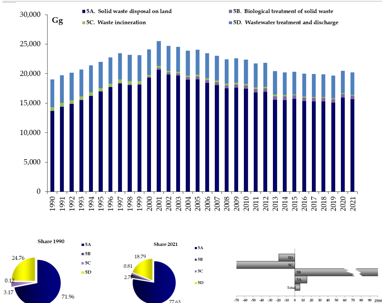
Figure 2.12 Trend of total emissions from the waste sector (1990-2021) (kt CO 2 eq.)
