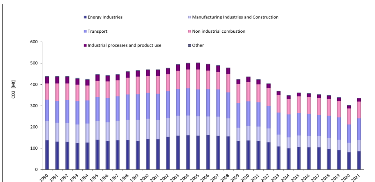
Figure 2.3 National CO 2 emissions by sector from 1990 to 2021 (Mt)
