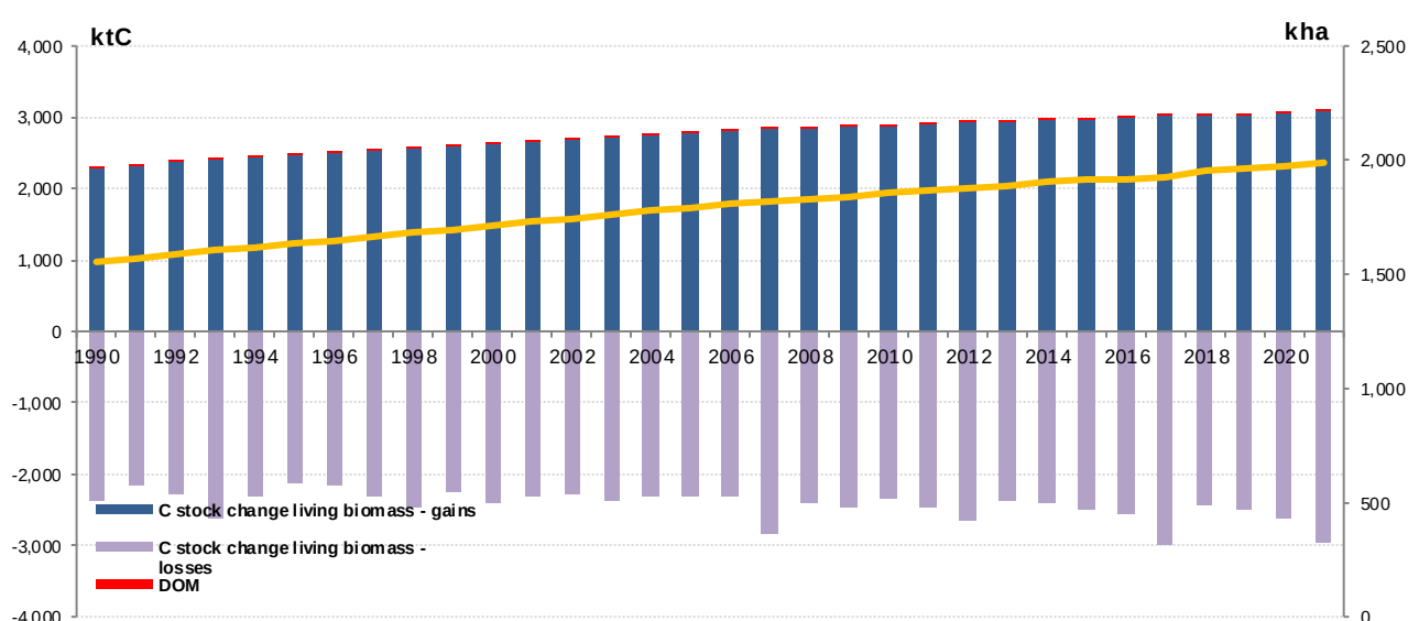
Figure 6.9 Other wooded land areas and net changes in carbon stock, for the different pools
