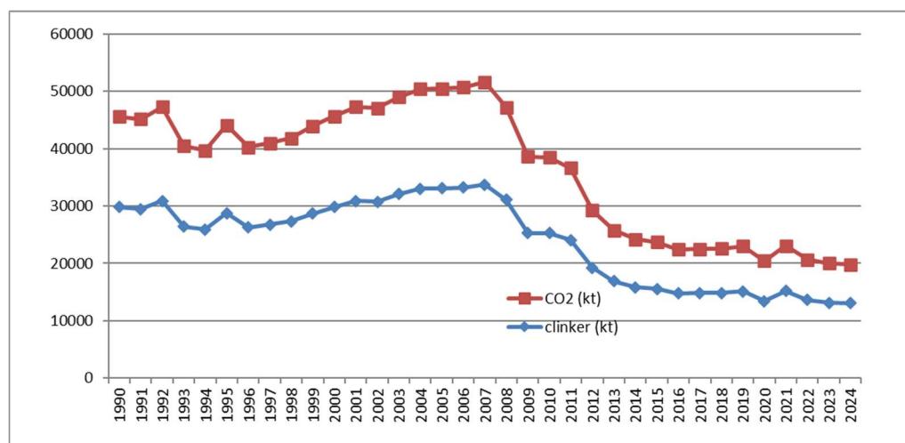
Figure 4.2 Trend of clinker production and CO 2 emissions 1990-2024 (kt)
