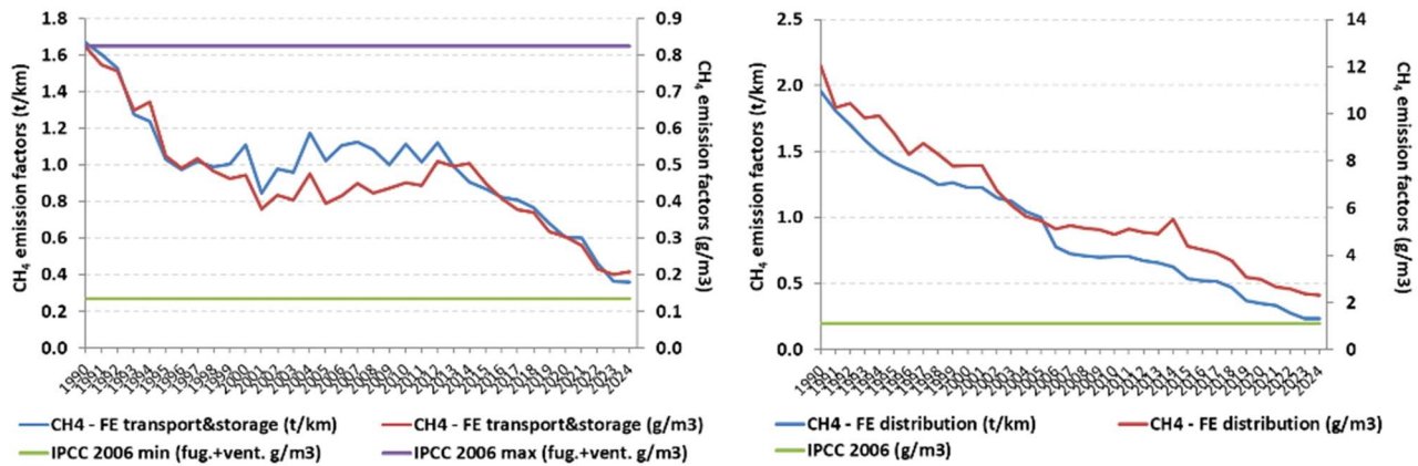
Figure 3.2 Trend of \text{CH}_4 emission factors for natural gas transmission and distribution compared with the respective default EFs (IPCC, 2006).
