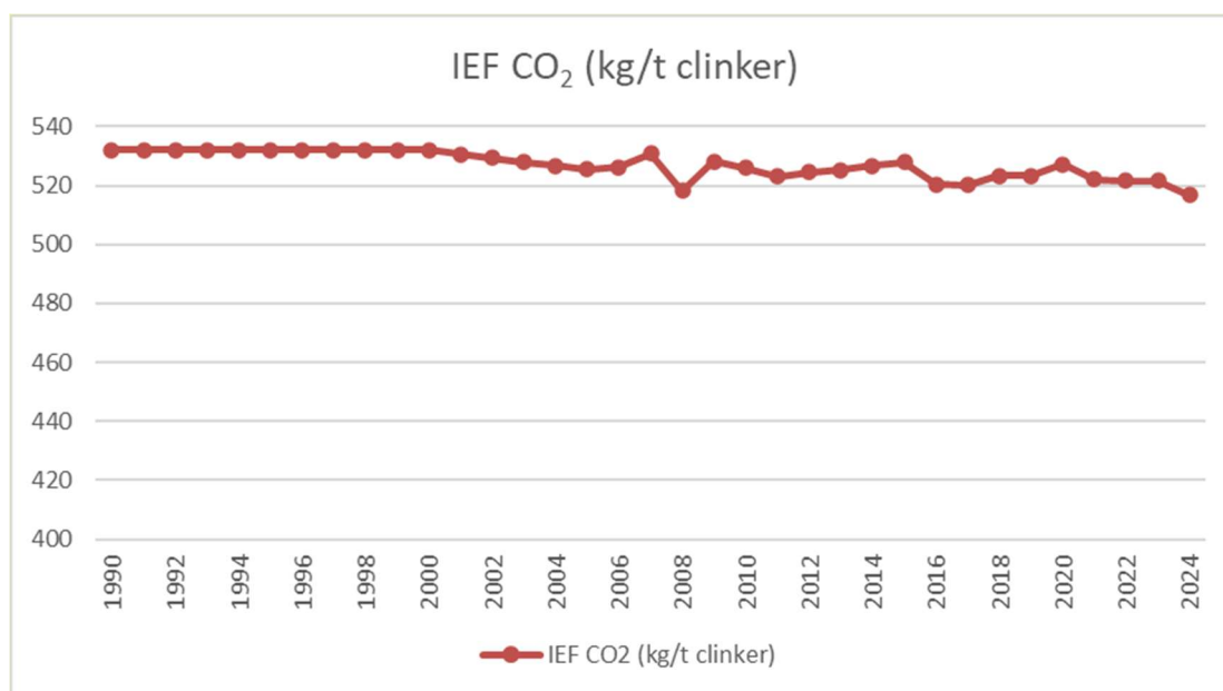
Figure 4.1 CO 2 IEF from decarbonation in clinker production, 1990-2024
