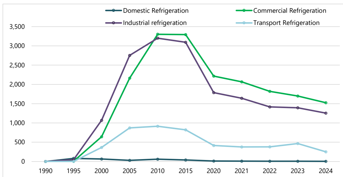
Figure 4.3 Total HFC emissions by sub-sector of refrigeration sector (ktCO 2 eq), 1990-2024
